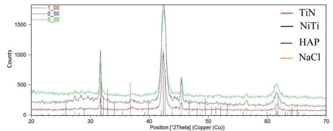
Fig. 8. GIXD patterns measured at incidence angle of 0.3° for the nitrided NiTi alloy with deposited hydroxyapatite layer
