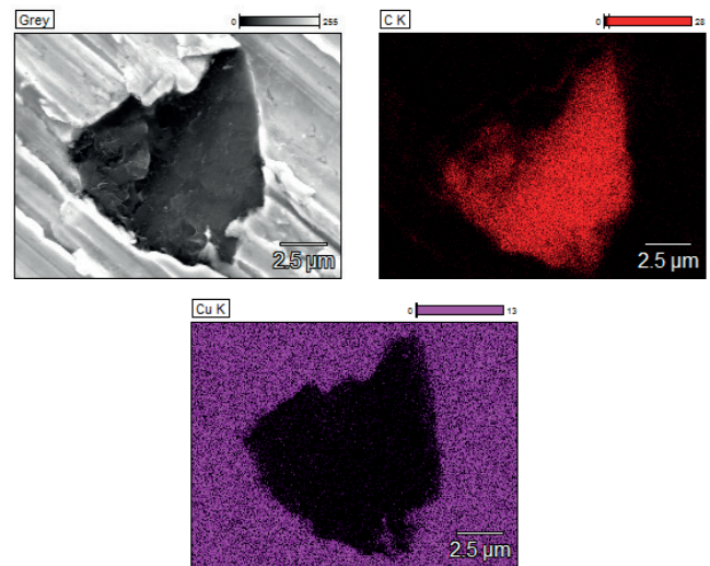
Fig. 3. Distribution of copper and carbon elements in the hole
