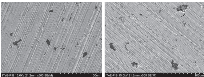
Fig. 1. SEM images of the composite surfaces with the distribution of graphene oxide particles. Visible microcraters in the matrix material
