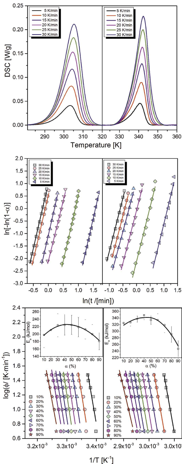
Fig. 7. Complex analysis of structural transition kinetics in Samples 1 and 3 with different Ge/P ratios. Top panel – DSC curves for different heating rates, middle panel – Avrami fits of kinetic curves, bottom panel – FWO fits and activation energies.
