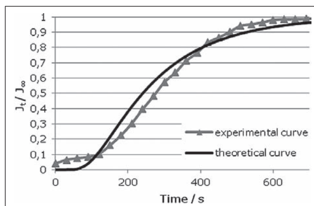
Figure 5 Fitting the experimental data with the theoretical curve for the 2 nd BUT after 5% tensile deformation
