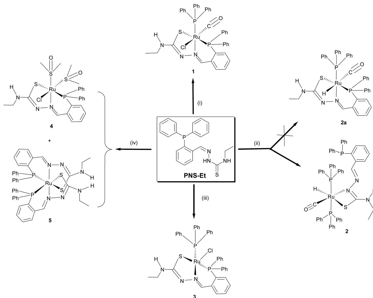
Scheme 3 Synthesis of ruthenium(II) complexes (1–5). (i) [\text{RuHCl}(\text{CO})(\text{PPh}_3)_3] , \text{C}_2\text{H}_5\text{OH} , reflux 8 h (ii) [\text{RuH}_2(\text{CO})(\text{PPh}_3)_3] , \text{C}_2\text{H}_5\text{OH}/\text{CH}_2\text{Cl}_2 , reflux 12 h (iii) [\text{RuCl}_2(\text{PPh}_3)_3] , \text{C}_2\text{H}_5\text{OH}/\text{CH}_2\text{Cl}_2 , reflux 8 h (iv) \text{cis-}[\text{RuCl}_2(\text{Me}_2\text{SO})_4] , \text{C}_2\text{H}_5\text{OH} , reflux 12 h.
