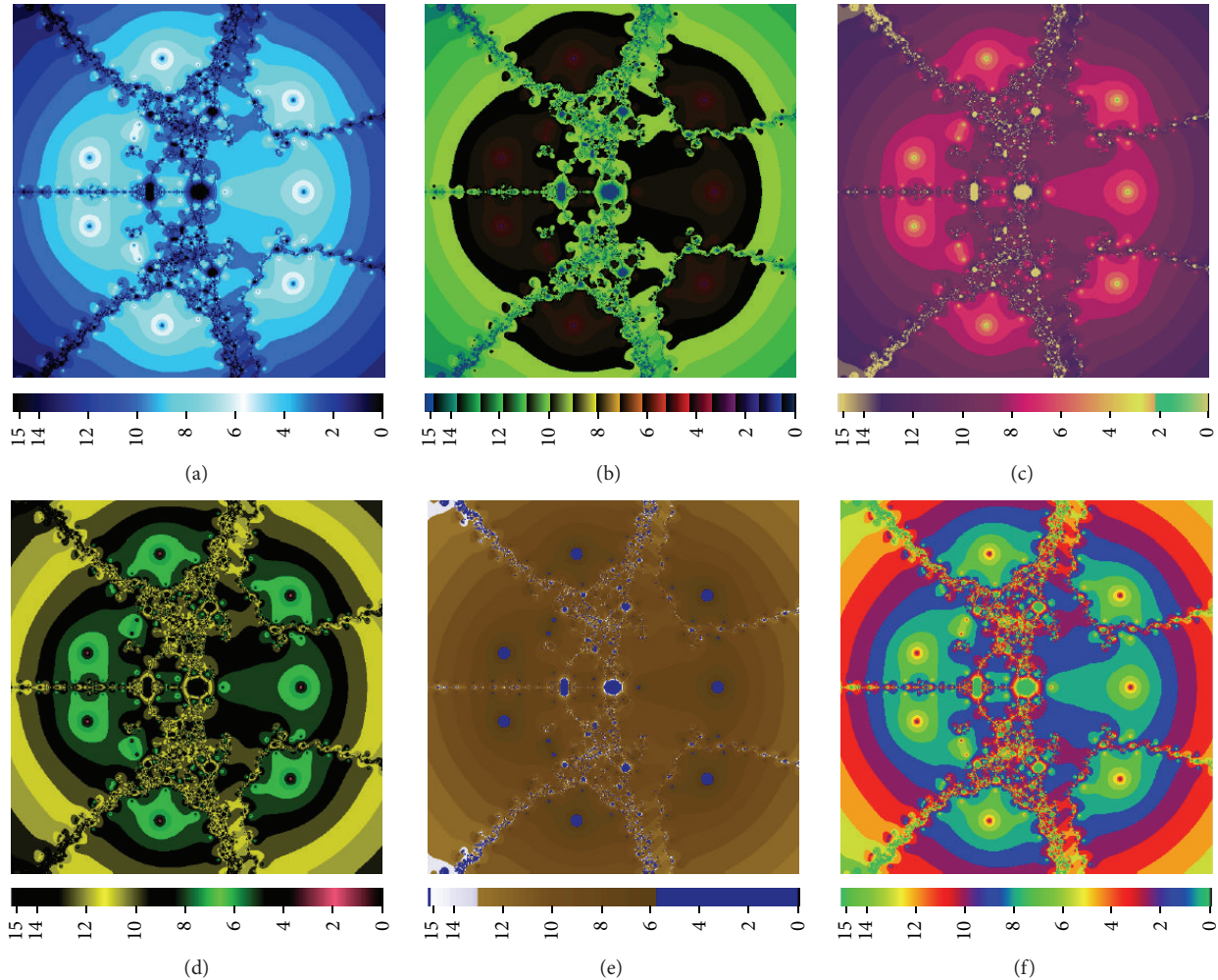
FIGURE 8: Examples of different colour maps application for the fixed polynomiograph.
