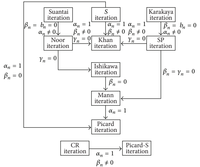
FIGURE 1: The diagram of iterations' dependencies.
