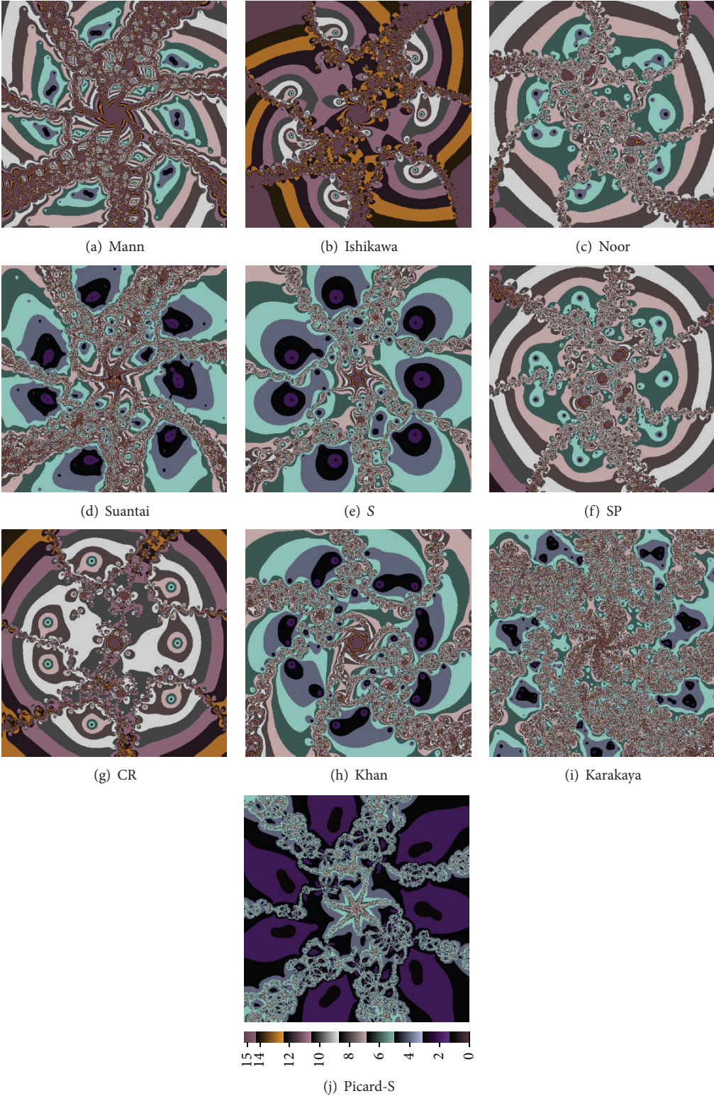
FIGURE 4: Examples of polynomiographs for p_1 with complex-valued parameters of iterations.
