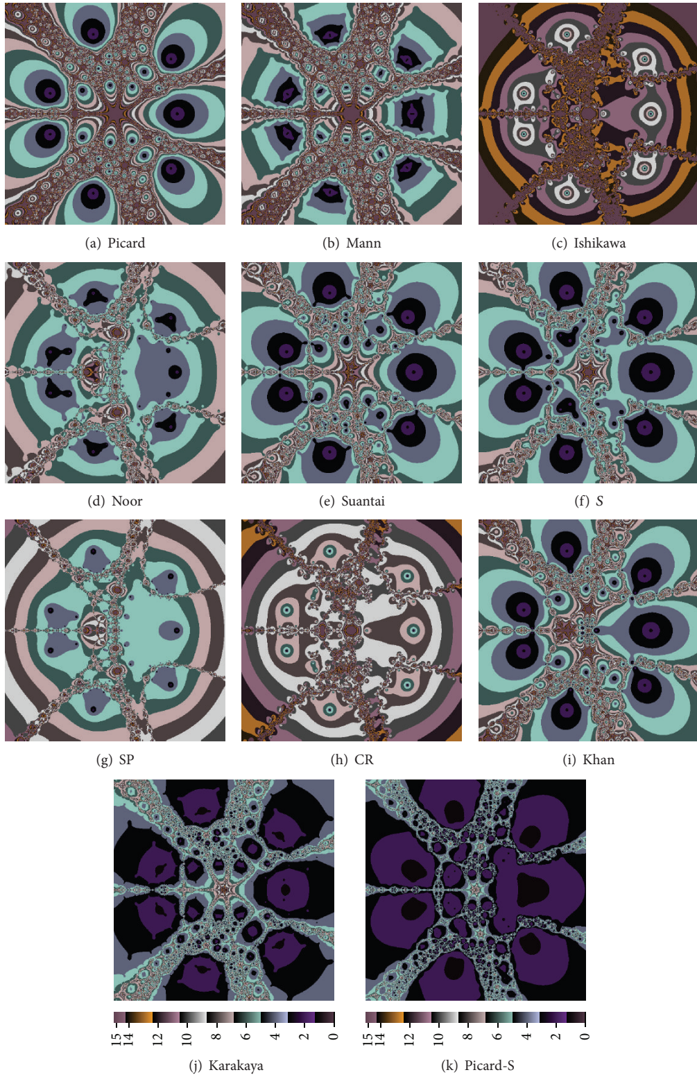
FIGURE 2: Examples of polynomiographs for p_1 with real-valued parameters of iterations.
