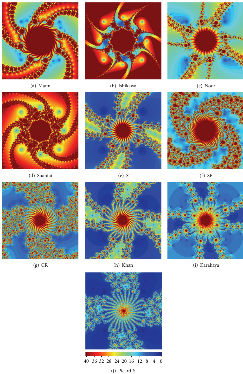
FIGURE 5: Examples of polynomiographs for p_1 with complex-valued parameters of iterations.
