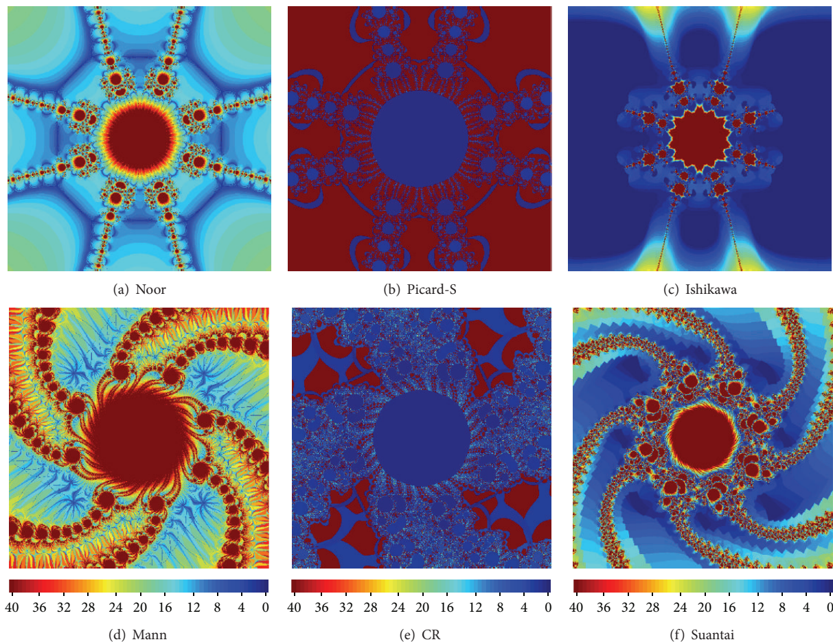
FIGURE 7: Examples of different convergence tests application for p_2 , the iterations with: real-valued parameters (a, b, and c) and complex-valued parameters (d, e, and f).
