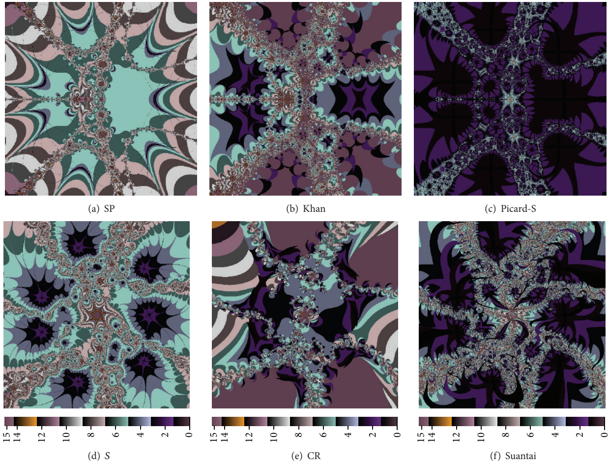
FIGURE 6: Examples of different convergence tests application for p_1 , the iterations with: real-valued parameters (a, b, and c) and complex-valued parameters (d, e, and f).
