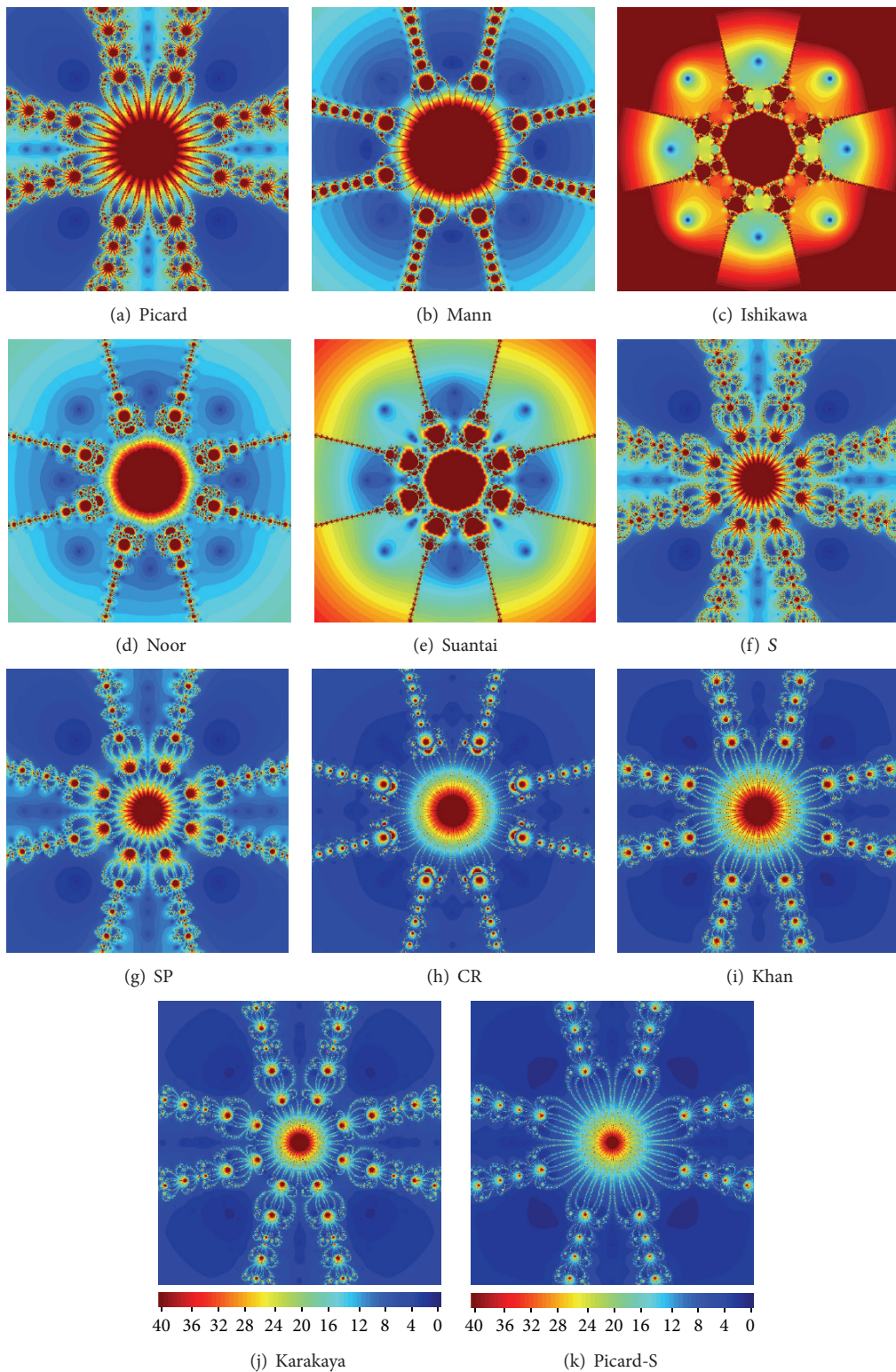
FIGURE 3: Examples of polynomiographs for p_2 with real-valued parameters of iterations.
