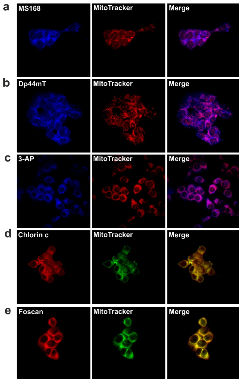
Fig. 2. Cellular localization of TSCs; MS168 (a), Dp44mT (b), 3-AP (c) and PSs; chlorin c (d), Foscan (e) in the HCT116 cell line. First panel – fluorescence of the investigated compounds alone, middle panel - colocalization with mitochondria marker (MitoTracker® Orange for TSC's and Green for PS's), last panel - merge. Scale bar represents 50 \mu\text{m} .
