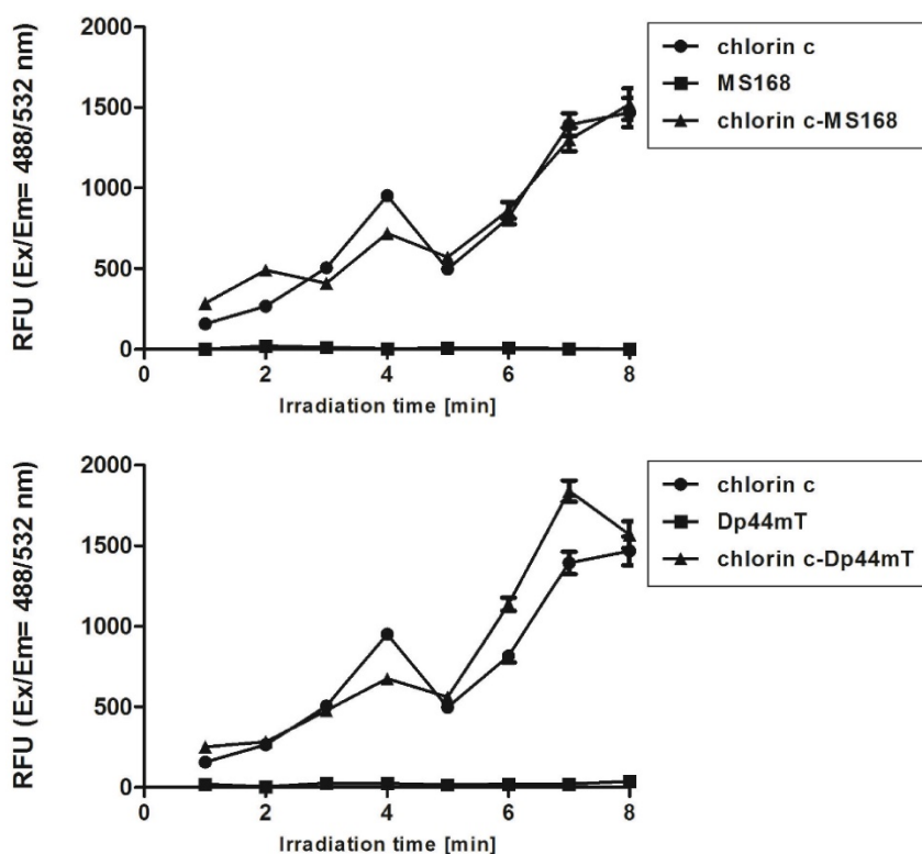
Figure A . Fluorescence response of the Singlet Oxygen Sensor Green reagent to the ^1\text{O}_2 that was generated during the irradiation of DMEM solutions containing the investigated PSs and TSCs as well as their combinations. The duration of the irradiation that was applied corresponds to a light dose 4-32 J/cm 2 .
