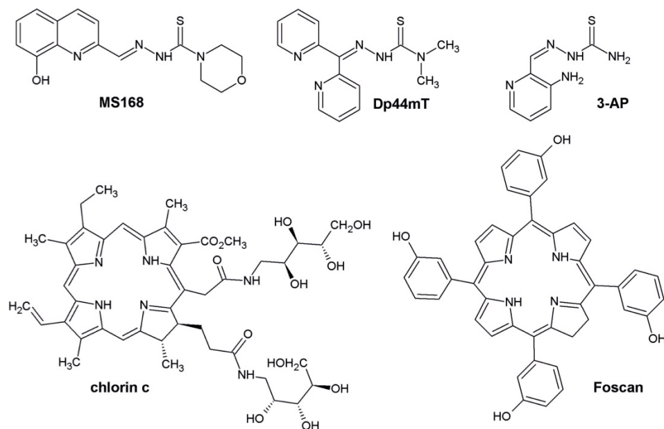
Fig. 1. Structures of TSCs ( MS168 , Dp44mT , 3-AP ) and PSs ( chlorin c , Foscan ).
