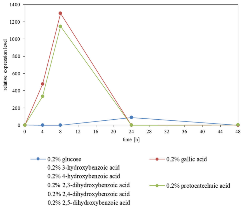
FIGURE 5 | Influence of carbon sources on the gene expression level of AGDC1 in A. adeninivorans G1212/YRC102 cultivated on YMM- \text{NaNO}_3 supplemented with each 0.2% glucose, gallic acid, protocatechuic acid, 3-hydroxybenzoic acid, 4-hydroxybenzoic acid, 2,3-dihydroxybenzoic acid, 2,4-dihydroxybenzoic acid and 2,5-dihydroxybenzoic acid. Expression analysis was performed by nested quantitative real time PCR.
