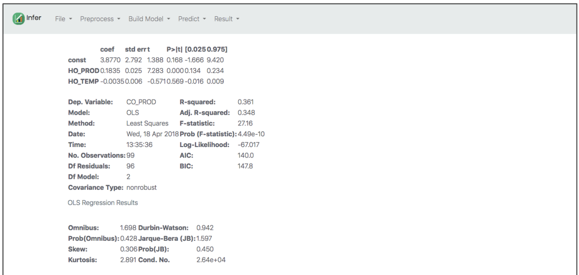
Figure 4.4: Linear regression model build with the new system.
