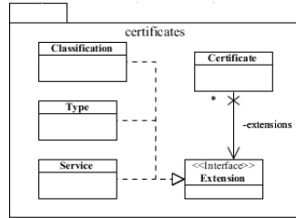
Fig. 2 Class diagram of the Certificate data structure.
