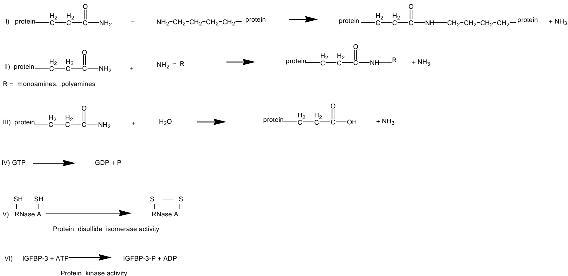
Figure 1. Examples of reactions catalyzed by TG: (I) acyl transfer between the \gamma -carboxamide group of a protein/polypeptide glutaminyl residue and the \epsilon -amino group of a protein/polypeptide lysyl residue; (II) attachment of a polyamine to the \gamma -carboxamide of a glutaminyl residue; (III) deamidation of the \gamma -carboxamide group of a protein/polypeptide glutaminyl residue; (IV) GTPase activity; (V) protein disulfide isomerase activity; (VI) protein kinase activity.
