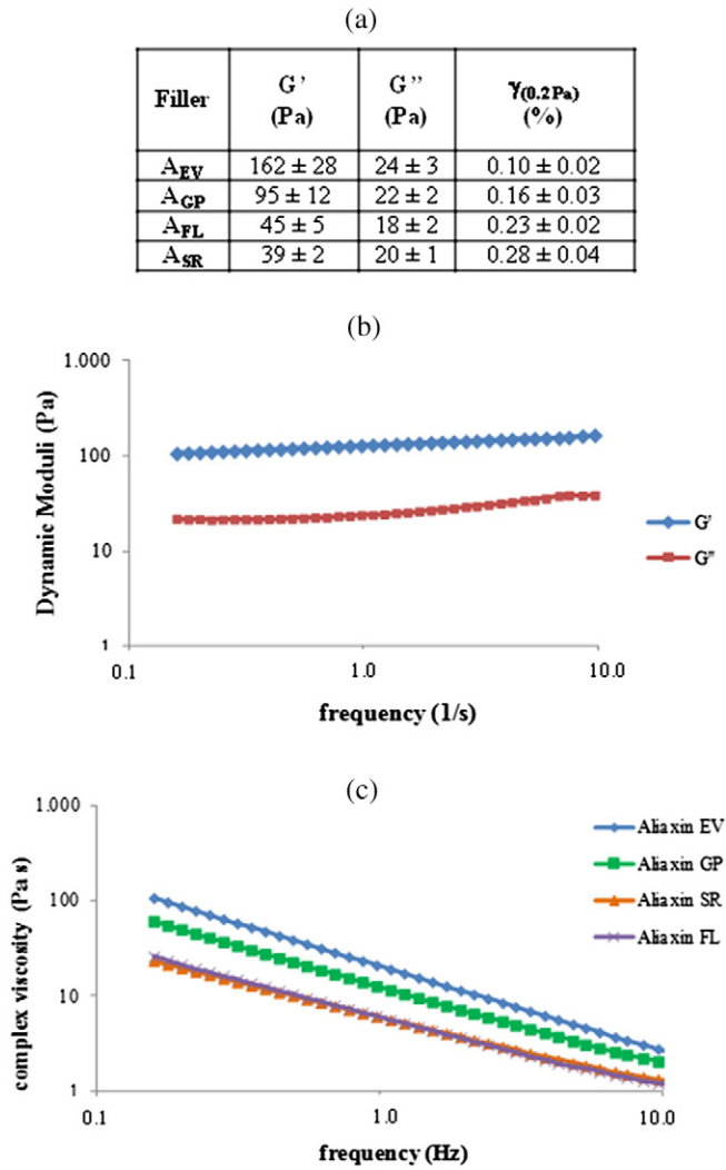
Fig. 1. (a) Storage modulus ( G' ), loss modulus ( G'' ), and strain values ( \gamma ) measured at 1.59 Hz frequency and 0.2 Pa stress (within the linear viscoelastic range) at 37 °C. (b) Aliaxin EV mechanical spectrum; (c) complex viscosity values, as obtained from the frequency sweep tests, as a function of frequency.
