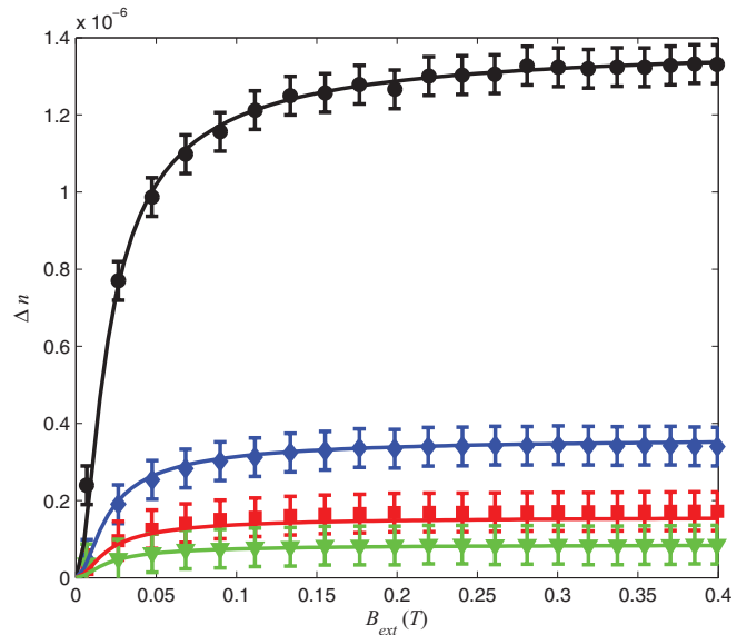
FIG. 1. (Color online) Birefringence ( \Delta n ) as a function of external magnetic field ( B_{\text{ext}} ) at different volume fractions ( f ) of the nanoparticles. Measurements at the maximum volume fraction are presented by circles; this concentration was diluted by factors of 2 (diamonds), 4 (squares), and 8 (triangles). The best fit to the data was obtained at \mu(2) = (1.4 \pm 0.1)\mu , where \mu = 6 \times 10^4 \mu_B is the value of the measured magnetic moment of a single nanoparticle. The wavelength of light is 633 nm.
