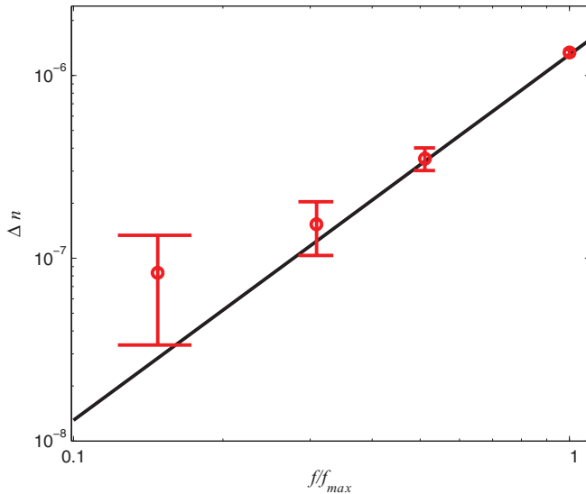
FIG. 2. (Color online) Measured birefringence ( \Delta n ) as a function of the relative volume fraction of nanoparticles ( f/f_{\max} ), where f_{\max} is the maximum volume fraction used in the experiments. The black line presents the dependence \Delta n \propto f^2 .
