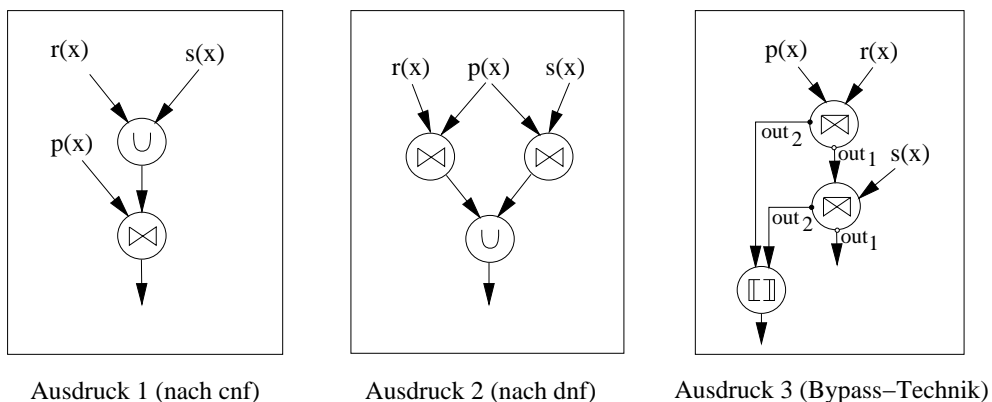
Abbildung 3: Motivation Bypass-Technik
