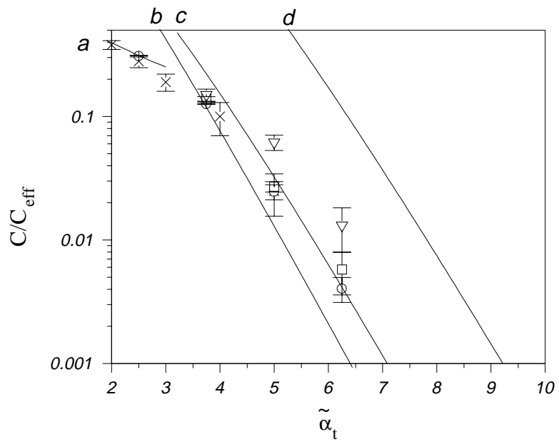
FIG. 8. The same data as in fig. 7 on a logarithmic scale.
