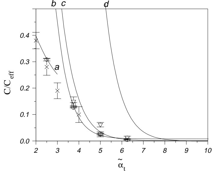
FIG. 7. Comparison between various theoretical predictions and Monte Carlo data for the renormalized capacitance C_{eff} in the strong tunneling regime \tilde{\alpha}_t \gtrsim 2 . The Monte Carlo data by Hofstetter and Zwerger [28] are denoted by crosses. The data obtained by Wang et al. [20] at E_C/T = 100, 200 and 500 are indicated respectively by circles, squares and triangles. At \tilde{\alpha}_t = 5 the data points [20] for E_C/T = 100 and 200 essentially coincide with that of [28]. The curve (a) shows the perturbative result by Grabert [11]. For all values of \tilde{\alpha}_t < 2 (not shown here) this result agrees well with the Monte Carlo data [20] and [28]. The curves (b), (c) and (d) indicate the results obtained by means of the instanton technique at sufficiently large \tilde{\alpha}_t : the results by Panyukov and Zaikin [18] obtained at sufficiently high T (the curve (b) – eqs. (52), (53)) and at T = 0 (the curve (c) – eq. (55) of this paper), as well as the T = 0 results by Wang and Grabert (eq. (10) of [21]).
