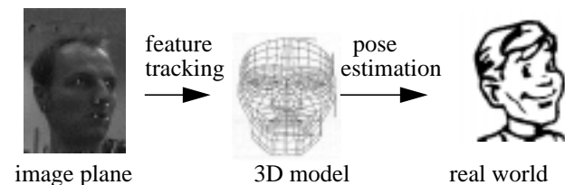
Figure 6. Gaze tracking as feature tracking + pose estimation
