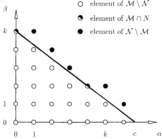
Figure 4: The sets \mathcal{M} and \mathcal{N} .
