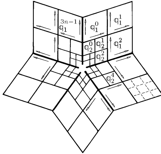
Figure 2: Subdivision surface around an extraordinary point.
