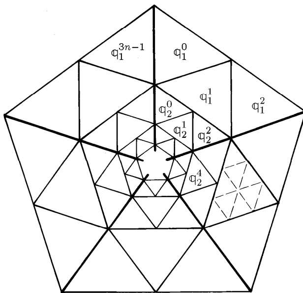
Figure 3: Subdivision surface with triangular control net around an extraordinary point.
