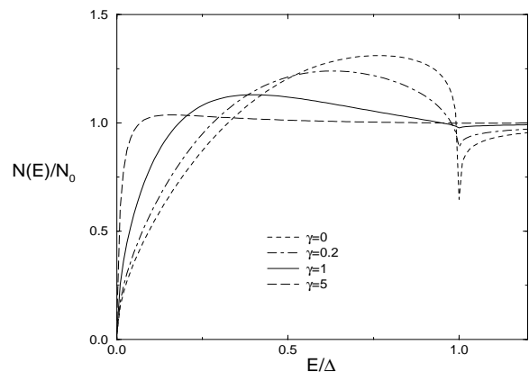
FIG. 2. DOS in the normal metal at x = 1.5\xi_n .
