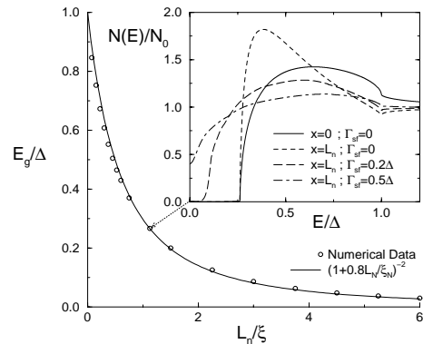
FIG. 5. Minigap E_g as a function of the normal-layer thickness. Inset: local DOS of an N-layer of thickness L_n = 1.1\xi in proximity with a bulk superconductor.
