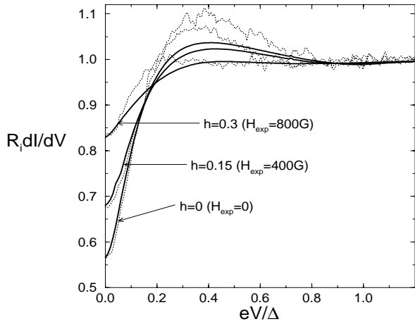
FIG. 7. Quantitative comparison of experiment 19 (dotted lines) and theory (solid lines). The experimental magnetic fields are H = 0, 400, and 800\text{G} ; h = HeW(D/12\Delta)^{1/2} . The theoretical curves have been normalized by R_i \equiv dI/dV_{\text{exp}}(eV/\Delta = 1.5) .
