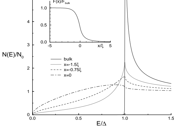
FIG. 3. Density of states on the superconducting side of the N-S boundary. The inset shows the self-consistent pair amplitude.
