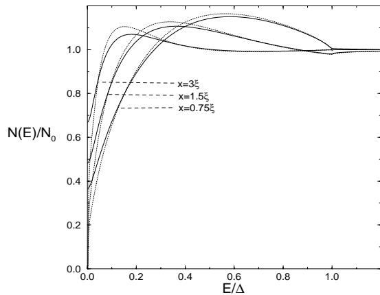
FIG. 4. Density of states on the normal side of an N-S boundary for two spin-flip scattering rates: \gamma_{sf} = 0 (dotted lines) and \gamma_{sf} = 0.015\Delta (solid lines).
