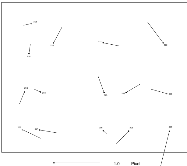
Figure 2: Residuals of Helmert transformation from slide-coordinates to the digitized image-coordinates on Pro Photo CD .
