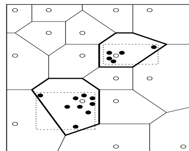
Fig. 1: approximated Voronoi regions
