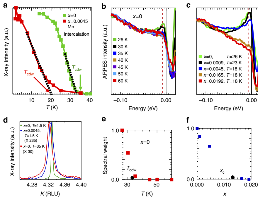
Figure 1 | CDW phase transition for pure and intercalated 2H\text{-NbSe}_2 samples. (a) Intensity of the CDW superstructure peak as a function of T for an x = 0 (green) and x = 0.0045 (Mn-intercalated, red). Dotted lines are guides to the eye, indicating the growth of the CDW order parameter. Arrows mark the estimated T_{\text{cdw}} which is the interpolation of the linear part to zero. (b) FF divided EDCs for various temperatures at the momentum location shown by the red dot in Fig. 2d. (c) FF divided EDCs for different x at the lowest measured temperatures. The sample with x = 0.0165 is intercalated with Co, the others are intercalated with Mn. The corresponding momentum location is shown by the pink dot in Fig. 2d. The red dashed line in b and c shows the energy location of the peak (for T < T_{\text{cdw}} and x < x_c ) and kink (for T > T_{\text{cdw}} or x > x_c ) in the EDCs, while the black line is the chemical potential. (d) Intensity profile of CDW superstructure peaks along (0, K, 0) for x = 0, 0.0045 (intercalated with Mn) at 1.5 K and for x = 0 at T = 35 K. The intensities have been normalized to that of the (0, 4, 4) Bragg peak and have subsequently been multiplied by the factors displayed in the legend to make them all visible on the same scale. (e, f) Normalized spectral weight associated with the coherence peak, following the procedure as described below, as a function of T for x = 0 and as a function of x at the lowest measured temperature. The black dots correspond to T_{\text{cdw}} for x = 0 and x_c \sim 0.013 , respectively. For x = 0 , the coherent spectral weight was obtained as the remaining integrated spectral intensity after subtracting the highest measured temperature (60 K) as background and dividing by the value obtained at the lowest measured temperature. We adopt the same procedure, as for the normalized spectral weight as a function of T , for its x dependence by considering the spectrum at the highest value of x as the background and dividing the coherent spectral weight at the lowest measured temperature for each x by the one for x = 0 .
