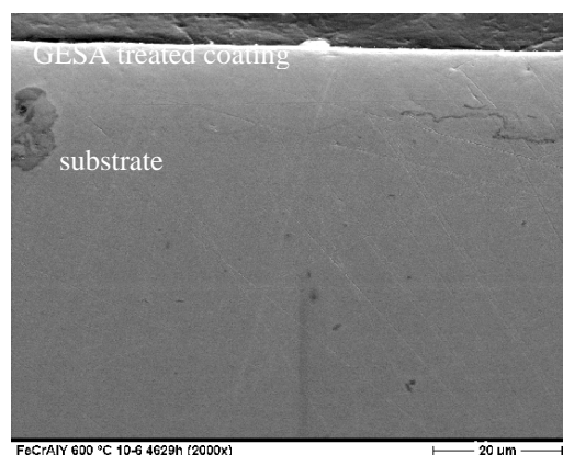
Fig. 1. Cross section of 1,4970 GESA [12] alloyed steel tested in flowing HLM at 600°C for 5000h.
