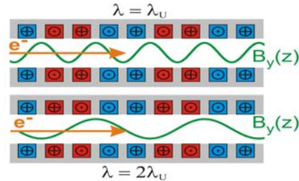
Figure 1: Sketch of the principle of period length switching (period doubling).
