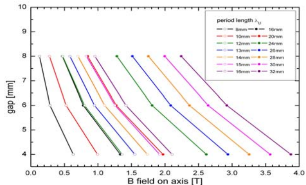
Figure 3: Gap versus K value (left plot) and gap as a function of the maximum B field on axis (right plot). Each for different period lengths.
