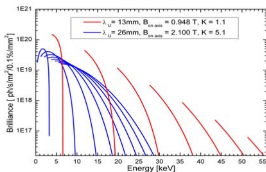
Figure 4: Brilliance plotted against photon energy.
