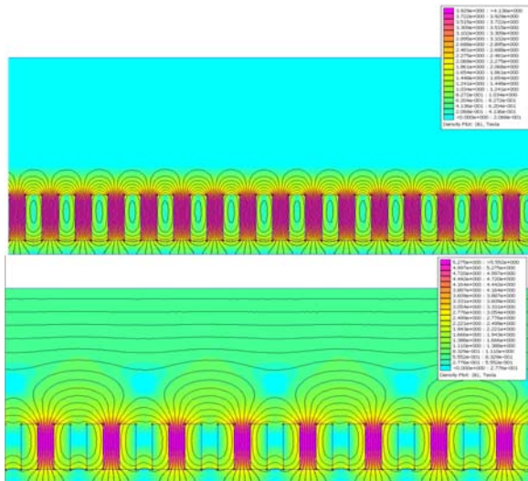
Figure 2: 2D coloured magnetic density plot for a gap of 8mm, \lambda_U = 14 mm (fundamental on top) and \lambda_U = 28 mm (doubled at bottom).
