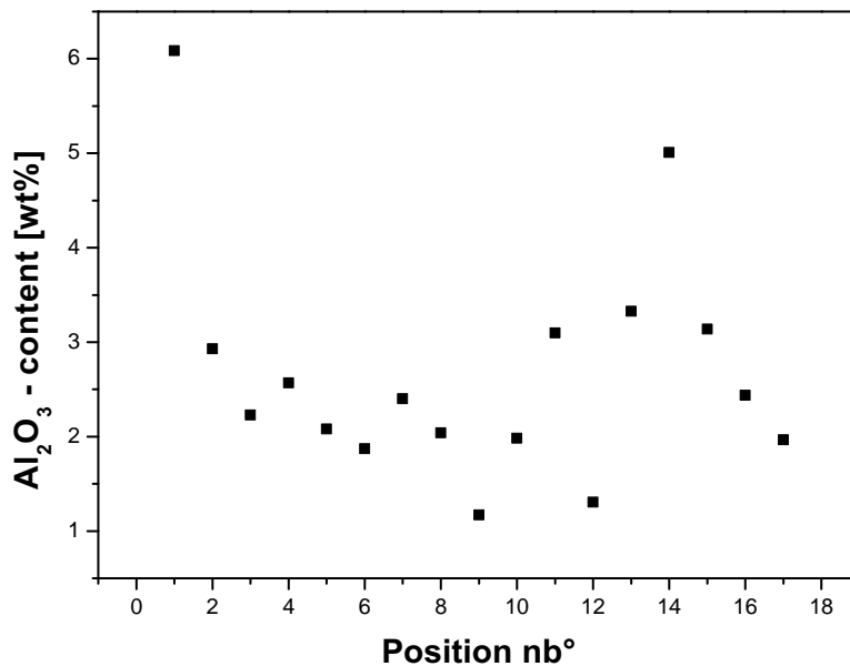
Figure 4.28: Al 2 O 3 content determined by point EDX-measurements on the cross section of the Ni-Al 2 O 3 microspecimen presented in Figure 4.27.
