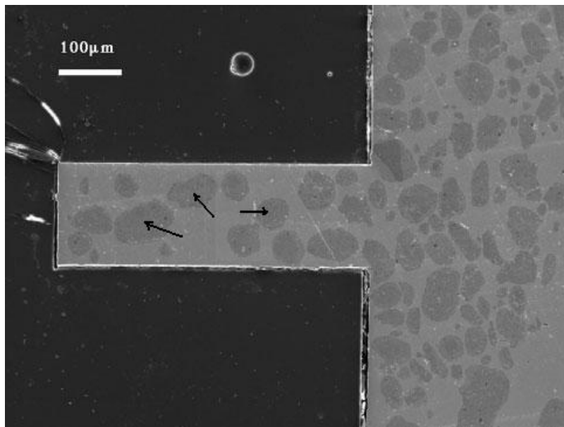
Figure 2.5: SEM cross sectional micrograph of a \text{Ni-Al}_2\text{O}_3 post grown from a bath containing 25 \text{ g l}^{-1} \text{Al}_2\text{O}_3 particles: particles agglomerates in both post and overplated layer [51]. Several \text{Ni-Al}_2\text{O}_3 agglomerates are indicated by arrows.
