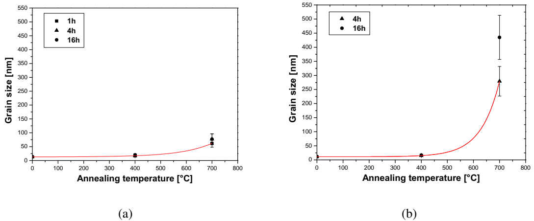
Figure 4.13: Dependence of the grain size determined by XRD on the annealing temperature: a- for Ni 15 at% W annealed at different durations (1h, 4h, 16h), b- for Ni 5 at% W annealed at different durations (4h, 16h).
