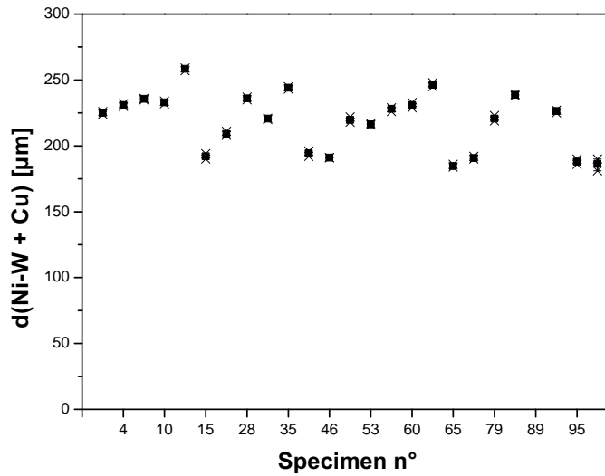
Figure 4.6: Thickness distribution of the electrodeposited material on the wafer surface. The thickness is the sum of Ni 5 at% W and 10 \mu\text{m} thick sacrificial copper layer.
