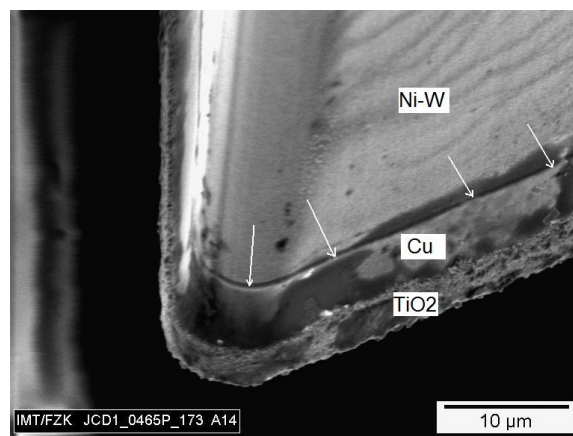
Figure 4.7: Lower part of a microspecimen profile including Ni-W, sacrificial Cu and \text{TiO}_2 . A step between Cu and Ni-W is indicated by arrows.
