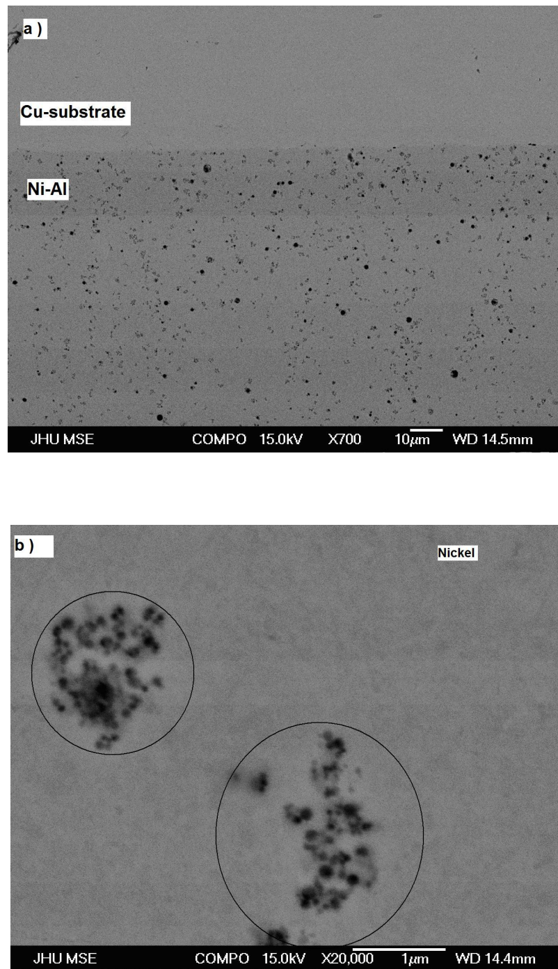
Figure 4.43: SEM-images of the NiAl 1 (see Table 4.9) cross section at different magnifications (a, b) [106]. The layer is attached to the copper substrate. Several aluminum agglomerates are illustrated inside circles (b).
