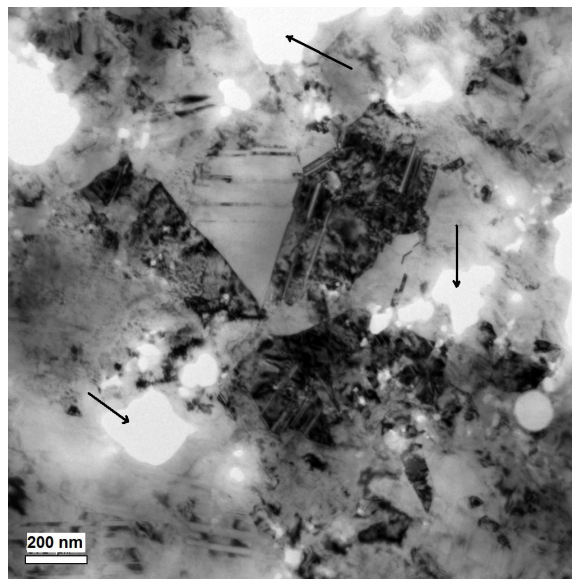
Figure 4.35: TEM-image of a Ni- \text{Al}_2\text{O}_3 TEM-disk electrodeposited according the parameters used to electrodeposit the microspecimens shown in Figure 4.29. The arrows indicate several voids.
