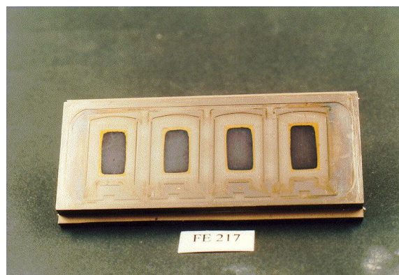
Figure 2.3: LIGA mold insert (Ni) for the fabrication of a commercially available microspectrometer (Boehringer Ingelheim - MicroParts, Germany). A batch of four microspectrometers can be fabricated during a single hot embossing step.
