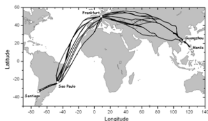
Fig. 1: CARIBIC flights from May 2005 to March 2007.
