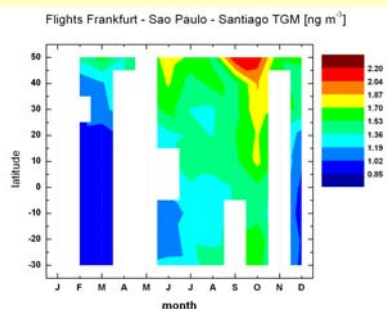
Fig. 2: Time latitude TGM distribution in the UT during the flights from Frankfurt to South America.
