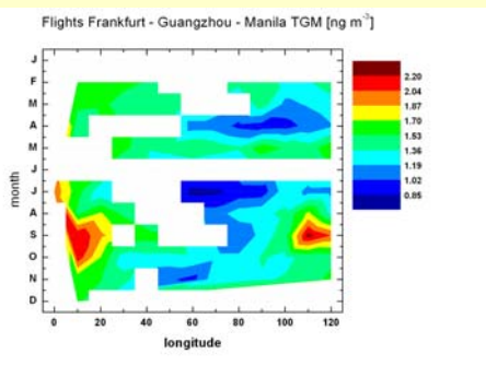
Fig. 3: Time longitude TGM distribution in the UT during the flights to Guangzhou and Manila
