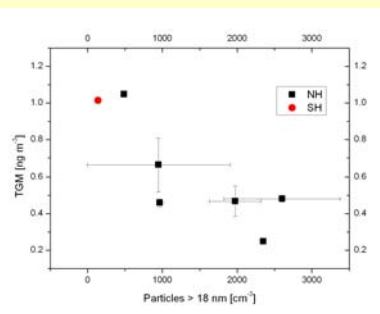
Fig. 6: The relation of stratospheric end point TGM concentrations to particle number concentrations.
