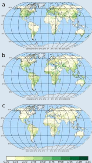
Modelled yields for wheat (a), maize (b) and rice (c) (Kg dry weight m -2 ). Hatching denotes model is within 1 \sigma of observations.
