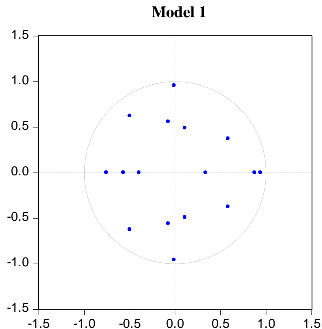
Figure 24: Inverse Roots of AR Characteristic Polynomial
