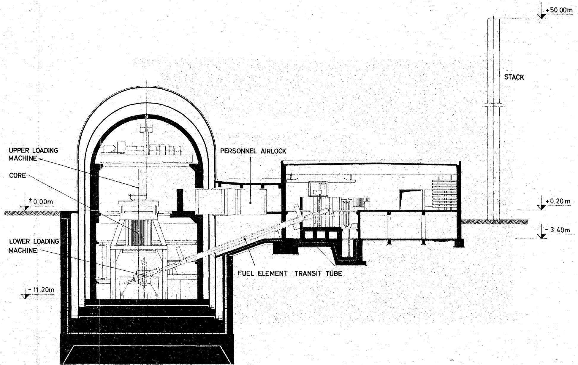
FIG. 2 SECTION THROUGH REACTOR BUILDING AND LOADING AREA
