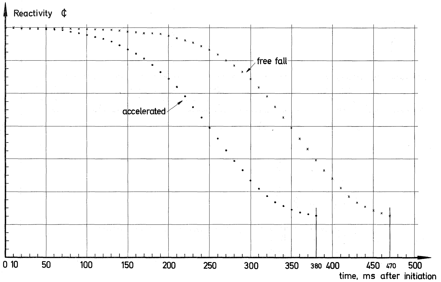
FIG. 8 REACTIVITY REDUCTION VS. TIME AT REMOVAL OF SAFETY ROD NO. 12, SNEAK 3A-1
