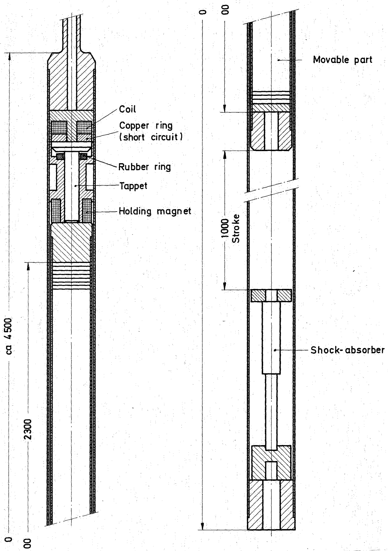
FIG. 7 SAFETY ROD
