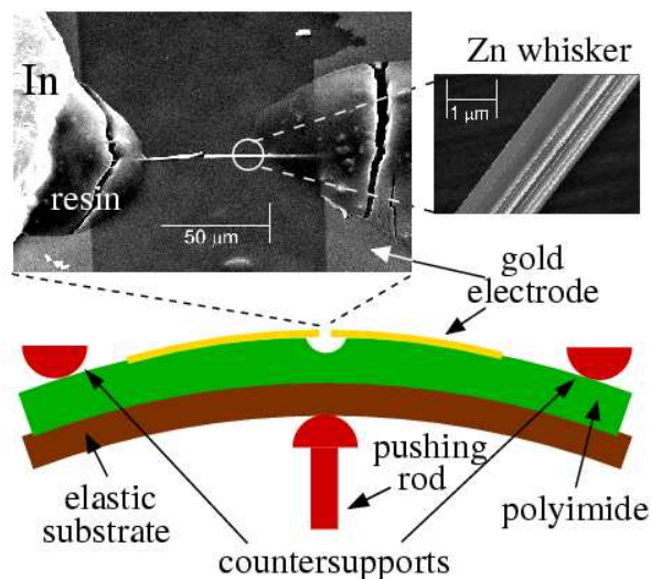
FIG. 1: (Color online) Three-point bending mechanism. The pushing rod bends the bronze substrate. The optical micrograph shows a whisker MCB after measurement. Right inset: blow up of a typical Zn whisker with a diameter of 1.7 \mu\text{m} .
