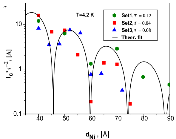
FIG. 2: The critical Josephson current I_c as function of the Ni-layer thickness d_{Ni} . The solid line shows the theoretical curve with E_{ex} = 200 meV used as a fitting parameter. The dots are the experimental data.
