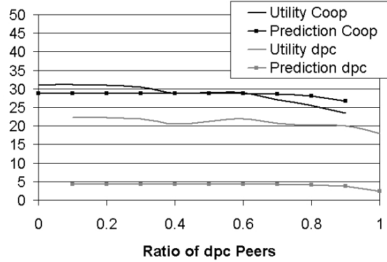
Figure 2. Influence of dpc peers.
