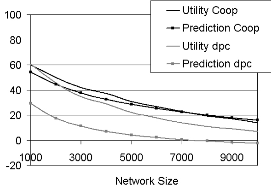
Figure 4. Influence of network size.
