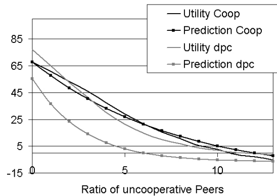
Figure 3. Influence of uncooperative peers.
