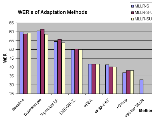
Figure 3: WER's of Adaptation Methods
