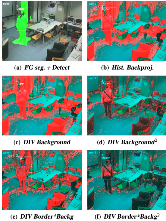
Figure 4: Improving color histograms. a ) shows the results of foreground segmentation (in green ) and object detection ( white rectangle ). The foreground pixels inside the rectangle are used to create the person’s color histogram. b ) shows the results of histogram backprojection. Red means high probability of belonging to the person, blue means low probability. c ), d ), e ) and f ) show the effect of different types of histogram division. Background stands for the general background histogram. Border stands for the histogram of the background region immediately surrounding the person
