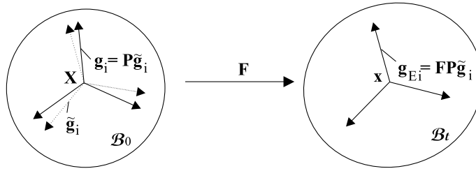
Fig. 1. The deformation gradient \mathbf{F} maps material tangent vectors from the reference placement of the body \mathcal{B}_0 to the current placement \mathcal{B}_t . The inelastic transformation \mathbf{P} = \mathbf{g}_i \otimes \tilde{\mathbf{g}}_i maps the Lagrangian reference lattice vectors \tilde{\mathbf{g}}_i = \mathbf{g}_i(t=0) onto the current Lagrangian lattice vectors \mathbf{g}_i(t) . The Eulerian vectors are obtained by the mapping \mathbf{g}_{Ei} = \mathbf{F}\tilde{\mathbf{g}}_i . The transformation of the elasticity tensors follows the same rule (see Eq. (6)).
