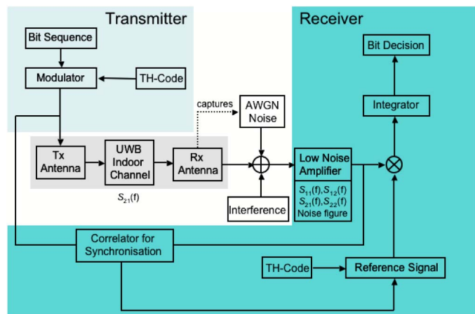
Fig. 1 System model of non-ideal UWB transmission
