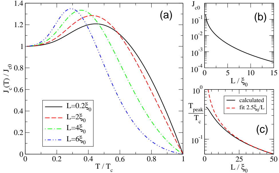
Fig. 5. (a) The normalized critical Josephson current density J_c(T)/J_{c0} as computed from Eq. (32) as a function of temperature T . The temperature dependence of the gap is given by the well-known BCS formula. (b) The zero temperature value J_{c0} = J_c(T = 0) is shown in units of eN_f v_f T_c |t_{\downarrow\uparrow}|^2 |t_{\uparrow\uparrow}|^2 \vartheta^2 as function of junction length L . (c) The peak position of the curves in (a) as function of L .
