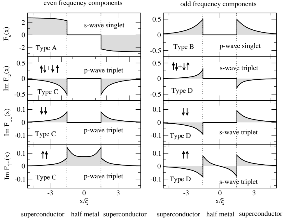
Fig. 3. Spatial dependences of all components of the pairing amplitude for a symmetric superconductor/half-metal/superconductor Josephson \pi -junction with interfaces characterized by the scattering matrix Eq. (27). The interfaces are indicated by the dashed lines. The components were numerically iterated until self consistency with the singlet order parameter was achieved. The interface parameters for normal impact angle are \vartheta = 0.3\pi , t_{\uparrow\uparrow} = 1 , t_{\downarrow\uparrow} = 0.7 , \vartheta_{\uparrow\uparrow} = \vartheta_{\downarrow\uparrow} = 0 , and the temperature is T = 0.2T_c .
