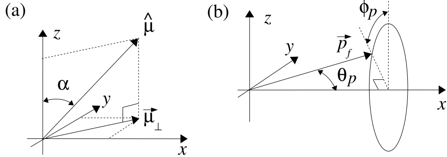
Fig. 1. (a) The spin quantization axis \hat{\mu} of the interface spin-active scattering matrix forms an angle \alpha with the exchange field in the ferromagnet and has a perpendicular component \vec{\mu}_{\perp} . (b) The direction of the momentum \vec{p}_f is expressed in spherical coordinates through the angles \theta_p and \phi_p .
