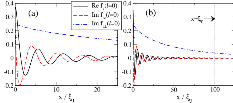
Fig. 2. Pair correlation functions in the ferromagnet of a ballistic superconductor-ferromagnet junction. The first partial wave ( l = 0 ) for the lowest Matsubara frequency, \epsilon_0 = \pi T , is shown. (a) For the singlet, f_s , and triplet with zero spin-projection on the exchange field, f_{tz} , we observe a 1/x -decay and oscillations, both on the scale \xi_J = v_f/2J . On the same scale the perpendicular triplet f_{t\perp} only varies slowly. (b) At large distances all components decay on the coherence length scale \xi_0 . However, the magnitudes of f_s and f_{tz} are considerably reduced compared with f_{t\perp} before this region is reached. We have chosen \xi_0 = 100\xi_J , \alpha = \pi/4 , \vartheta = \pi/4 , and we have normalized the functions by (\Delta/T)\sqrt{\mathcal{T}_+\mathcal{T}_-} .
