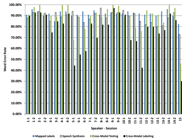
Figure 2: Word Error Rates per Speaker and Session for Different Recognizer Initialization Methods
