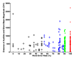
Figure 4: Utterance-based Absolute Deviation of EMG Channel 1 versus Word Error Rate
