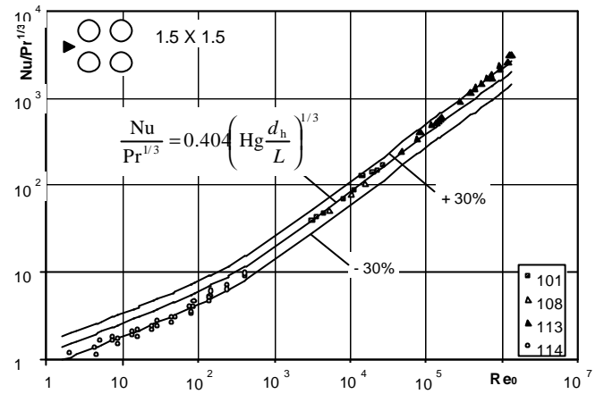
Fig. 2 Heat Transfer Group Nu/Pr^{1/3} vs. Reynolds-number, inline bundles a=1.5, b=1.5 , for the number of data sources (at the symbols) see Table 1. Hg=(\xi/2)Re_0^2 .
