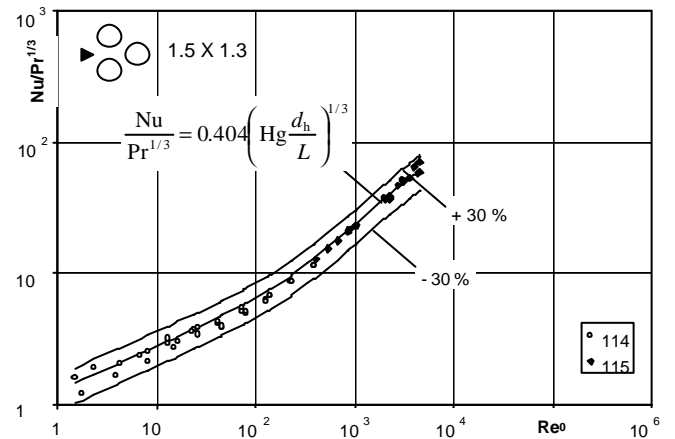
Fig. 4 Heat Transfer Group Nu/Pr^{1/3} vs. Reynolds-number, staggered bundles a=1.5, b=1.3 , for the number of data sources (at the symbols) see Table 1. Hg=(\xi/2)Re_0^2 .
