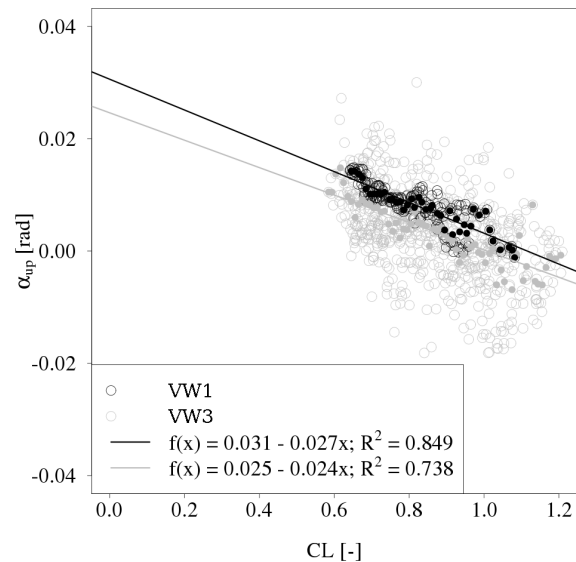
Fig. 9. Upwash attack angle ( \alpha_{up} ) as function of the lift coefficient ( CL ) for two vertical wind specific flight patterns on 25 June 2008 (VW1, VW3). \alpha_{up} is the difference of attack angle as measured by the five hole probe and the inverse reference of the free airstream attack angle (Sect. 4.1 Step G3). Open circles depict the entire 1 Hz dataset. Full circles are averages after binning over increments of 0.01 CL .
