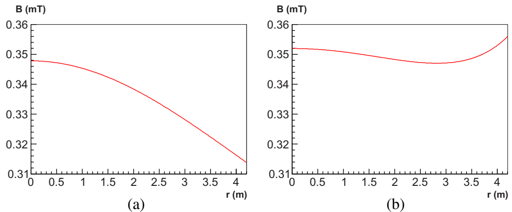
Figure 10. Magnetic field in the analyzing plane ( z = 0 ), as function of the radius. (a) One minimum field configuration and (b) two minima field configuration.
