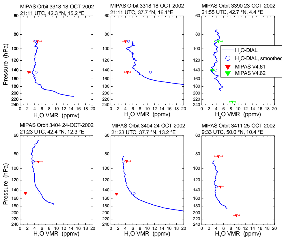
Fig. 10. Comparison of observed H 2 O-DIAL profiles (blue solid lines and circles) and MIPAS H 2 O data points version 4.61 (red triangles) and, in one case, version 4.62 (green triangles). H 2 O-DIAL profiles have been smoothed with the averaging kernel of MIPAS.
