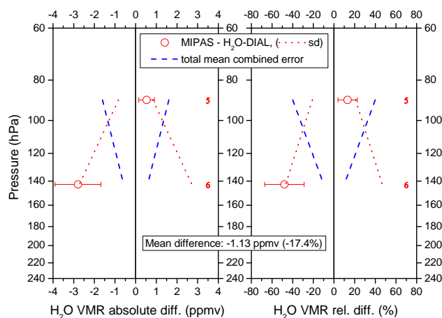
Fig. 11. Mean differences of all comparisons between MIPAS and smoothed H 2 O-DIAL observations (red circles) together with mean combined total errors (blue dashed lines) as well as standard deviation (red dotted lines) and the standard error of the mean, plotted as error bars. Red values indicate the number of collocations.
