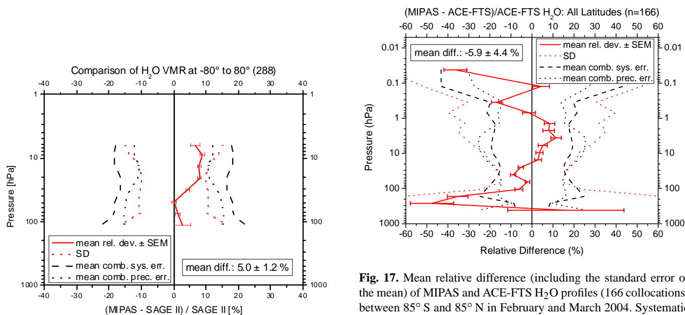
Fig. 16. Mean relative deviation of H 2 O profiles as measured by MIPAS and SAGE II for all collocations (288) between 80° S and 80° N. Annotation as per Fig. 13.
