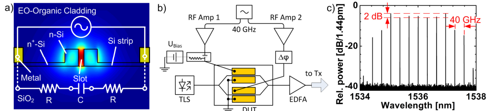
Fig. 1. Dual-drive frequency comb generator and spectrum. (a) Schematic cross-section and simulated optical mode of a silicon-organic hybrid (SOH) phase modulator. The two rails of a silicon slot waveguide are electrically connected to metal electrodes by 60 nm high n-doped silicon strips. The waveguide is covered by an electro-optic cladding material (DLD164), which entirely fills the slot. (b) Integrated dual-drive frequency comb generator: A tunable laser source (TLS) is coupled to a dual-drive SOH Mach-Zehnder modulator (MZM) via grating couplers. The arms are driven by two sinusoidal 40 GHz signals. Flat combs are obtained by carefully adjusting the signal powers and phases along with the bias voltage U_{\text{bias}} . Fiber-chip coupling losses are compensated by an erbium-doped fiber amplifier (EDFA). (c) Flat-top spectrum obtained for electrical drive powers of 28 dBm and 23 dBm measured at the output of the amplifiers, showing 7 lines within 2 dB flatness. The lines are spaced by 40 GHz.
