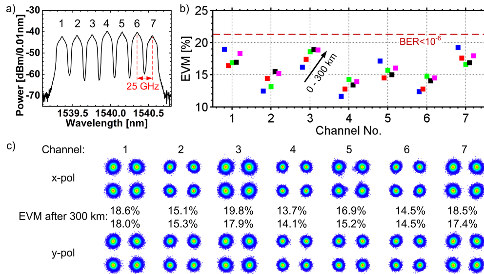
Fig. 5. Results for data transmission of QPSK signals: (a) Optical spectrum of the modulated carriers. The 7 strongest carriers are spectrally flattened by the WSS. (b) The average EVM of both polarizations over channel number are shown color-coded (and slightly offset for clarity of presentation) for each length of fiber span (0 km, 75 km, 150 km, 225 km, 300 km). Drift of the operation point of the integrated comb source leads to some deviations from equal optical power for each channel, but BER below 10^{-6} are achieved for all channels nonetheless. (c) Constellation diagrams of all 7 channels and both polarizations after 300 km transmission.
