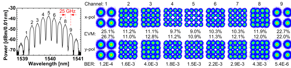
Fig. 4. Results of back-to-back data transmission. A total of 9 carriers spaced by 25 GHz were generated by an integrated SOH comb source. Optical spectrum of the modulated carriers (left) and constellation diagrams (right) for all channels and both polarizations are depicted along with measured EVM values. The 7 strongest carriers were modulated with Nyquist pulse-shaped 16QAM signals, whereas QPSK was used for weaker carriers 1 and 9. The symbol rate is 18 GBd. We obtain BER values below the hard-decision threshold for all channels, yielding an aggregate line rate of 1.152 Tbit/s.
