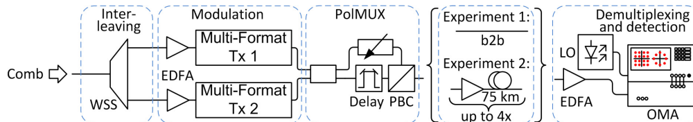
Fig. 3. Data transmission setup. A wavelength-selective switch (WSS) splits the comb into even and odd carriers which are modulated independently in a multi-format transmitter. The two sets of channels are recombined, and polarization multiplexing (PolMUX) is emulated by creating time-shifted copies of the data stream and merging them on orthogonal polarizations. Experiment 1: In a first experiment, the data is fed directly into the receiver (back-to-back, b2b). Experiment 2: Up to 4 spans of 75 km SMF are used for transmission over up to 300 km. At the receiver, the signal is amplified and the channels are demultiplexed and detected by an optical modulation analyzer (OMA). A free-running external cavity laser acts as a local oscillator (LO) for coherent reception.
