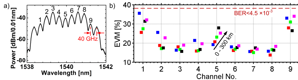
Fig. 6. Results for data transmission of NRZ QPSK signals: (a) Optical spectrum of the modulated carriers for 40 GHz spacing and 29 dBm of RF power measured at the output of the drive amplifier. (b) Average EVM of both polarizations over channel number. The results obtained for different fiber spans (0 km, 75 km, 150 km, 225 km, 300 km) are color-coded and slightly offset for clarity of presentation. Drift of the operating point of the comb source leads to variations of the BER obtained for different transmission distances. Nonetheless, BER values below the hard-decision threshold of 4.5 \times 10^{-3} are achieved for all channels, yielding a gross line rate of 1.008 Tbit/s.
