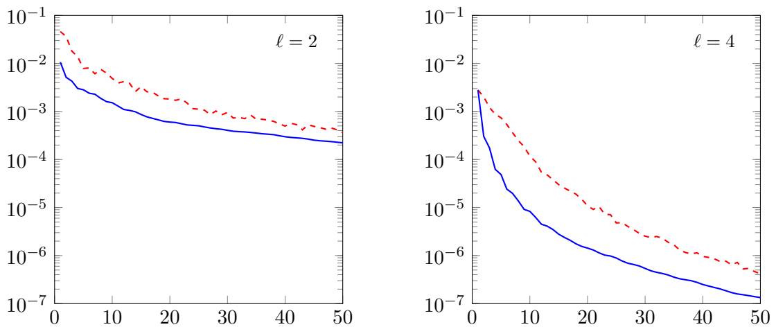
Figure 7.3: Comparison of the fixed rational approximation from Section 7.4 and the rational Krylov subspace approximation with simple poles. The errors \|\varphi_\ell(\mathbf{A})\mathbf{v} - \varphi_\ell(\mathbf{A}_m)\mathbf{v}\|_2 and \|\varphi_\ell(\mathbf{A})\mathbf{v} - S_m(\varphi_\ell, h, \mathbf{A})\mathbf{v}\|_2 are plotted versus m for \gamma = 2 , h = 0.5 , and \ell = 2, 4 .
