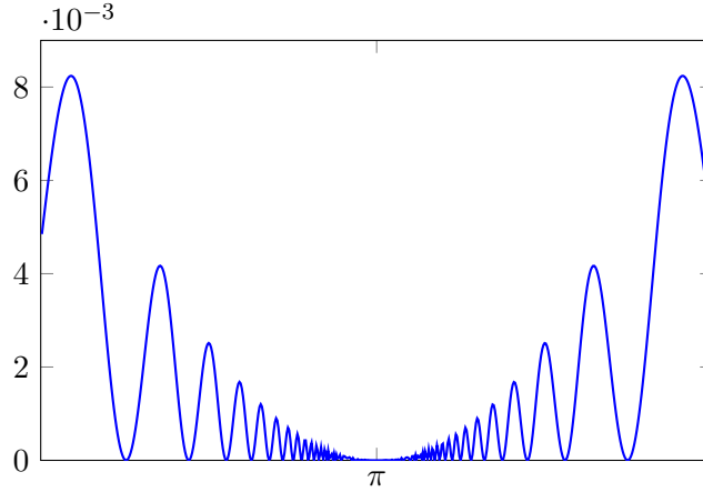
Figure 5.2: Plot of \text{Re}[\widehat{\varphi}_\ell(t)] for t \in [3, 3.28] , \ell = 2 , and \gamma = 1 .
