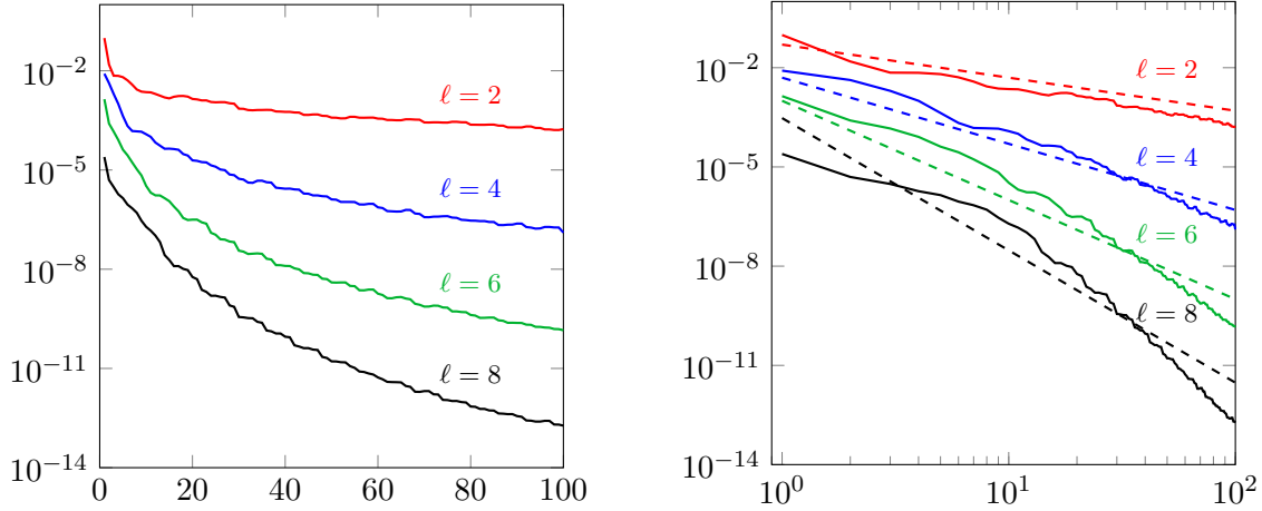
Figure 5.4: Left-hand side: Error \|\varphi_\ell(\mathbf{A})\mathbf{v} - \varphi_\ell(\mathbf{A}_m)\mathbf{v}\|_2 plotted against the number of shift-and-invert Krylov steps for \gamma = 1 . Right-hand side: Same plot as on the left but in double logarithmic scale together with lines of order \mathcal{O}(m^{-\ell/2}) , which correspond to the predicted convergence rate.
