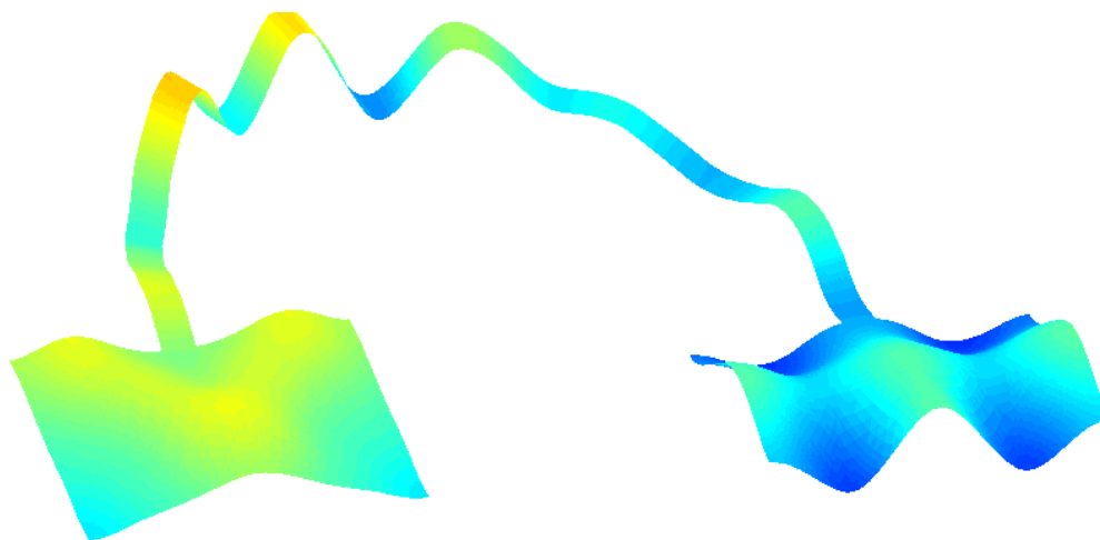
Figure 6.19: Approximation to the exact solution u at time \tau = 10 .
