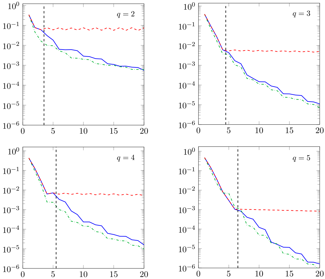
Figure 6.4: Plot of the error \|e^{\tau \mathbf{A}} \mathbf{y}_0^q - e^{\tau \mathbf{A}^{q+m}} \mathbf{y}_0^q\|_2 versus the dimension of the Krylov subspace for the standard Krylov subspace \mathcal{K}_{q+m,1}^\gamma(\tau \mathbf{A}, \mathbf{y}_0^q) (red dashed line), the rational Krylov subspace \mathcal{K}_{1,q+m}^\gamma(\tau \mathbf{A}, \mathbf{y}_0^q) (green dash-dotted line), and the extended Krylov subspace \mathcal{K}_{q+1,m}^\gamma(\tau \mathbf{A}, \mathbf{y}_0^q) (blue solid line) with initial vectors \mathbf{y}_0^q , q = 2, 3, 4, 5 , whose continuous counterparts satisfy y_0^q \in D(A^q) but y_0^q \notin D(A^{q+1}) . The parameters are chosen as \gamma = 1 , \tau = 0.1 , and N = 1023 .
