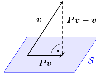
Figure 4.1: Orth. projection of \mathbf{v} onto the subspace \mathcal{S} .
