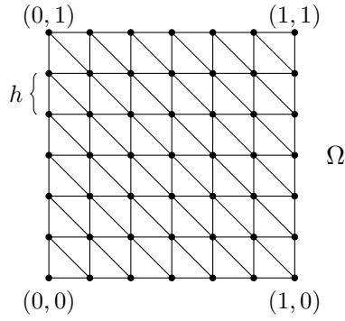
Figure 6.6: Regular triangulation of the unit square together with the used (n + 2)^2 grid nodes of the finite-difference and the finite-element discretization.
