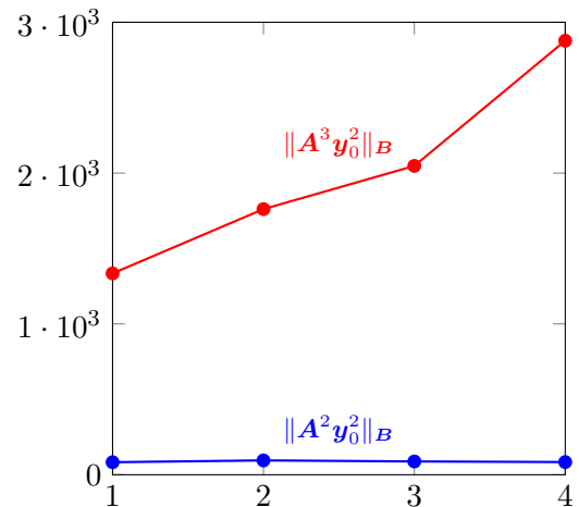
Figure 6.14: Values \|\mathbf{A}^j \mathbf{y}_0^2\|_B , j = 2, 3 , for different refinements of the mesh.
