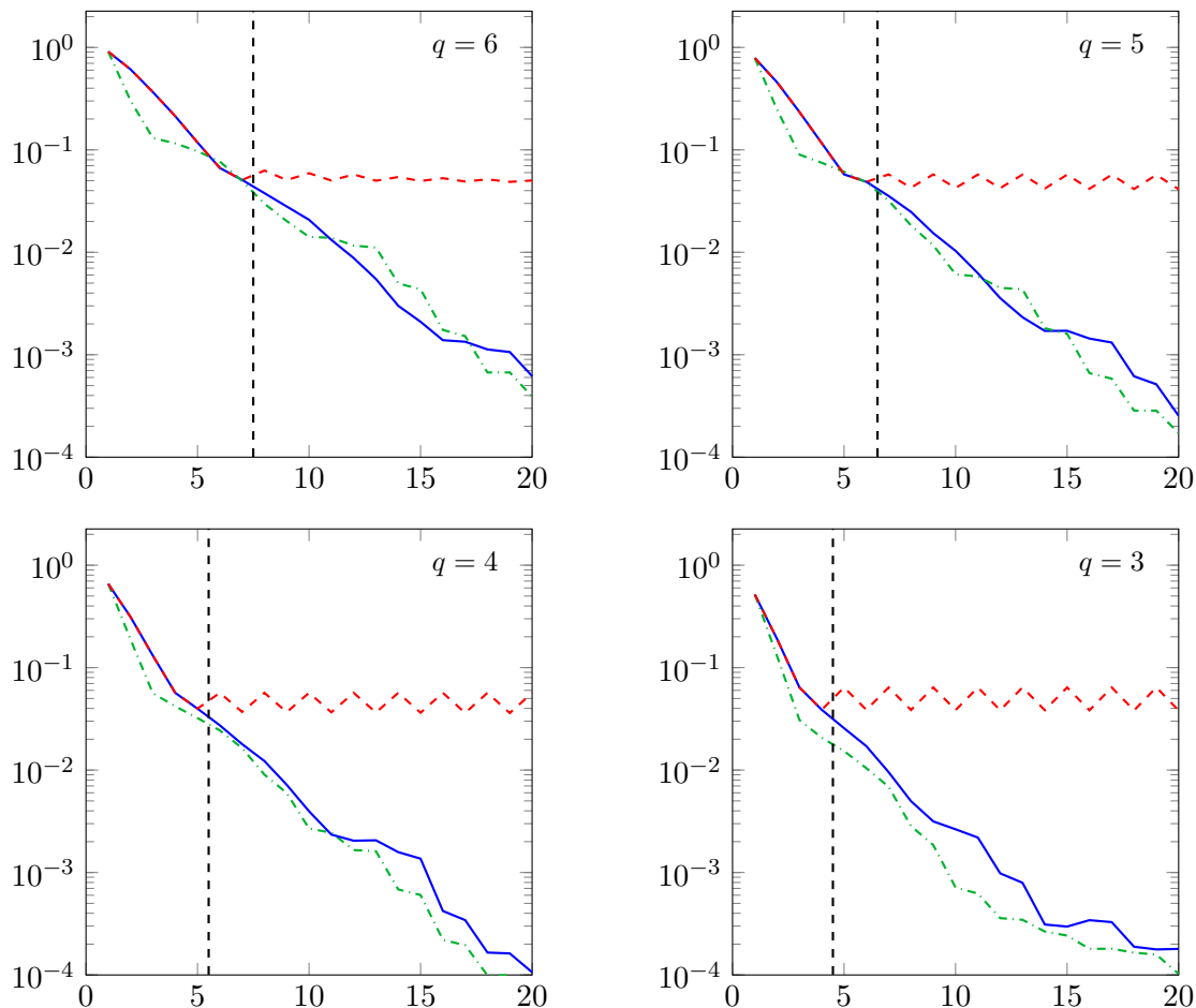
Figure 6.7: Plot of the error \|e^{\tau \mathbf{A}} \mathbf{y}_0^q - e^{\tau \mathbf{A}_{q+m}} \mathbf{y}_0^q\|_M versus the dimension of the Krylov subspace for the standard Krylov subspace \mathcal{K}_{q+1,m}^\gamma(\tau \mathbf{A}, \mathbf{y}_0^q) (red dashed line), the rational Krylov subspace \mathcal{K}_{1,q+m}^\gamma(\tau \mathbf{A}, \mathbf{y}_0^q) (green dash-dotted line) and the extended Krylov subspace \mathcal{K}_{q+1,m}^\gamma(\tau \mathbf{A}, \mathbf{y}_0^q) (blue solid line) for N = 16\,129 , q = 6 (top left), N = 65\,025 , q = 5 (top right), N = 261\,121 , q = 4 (bottom left), N = 1\,046\,529 , q = 3 (bottom right), and parameters \gamma = 1 , \tau = 0.005 in each case.
