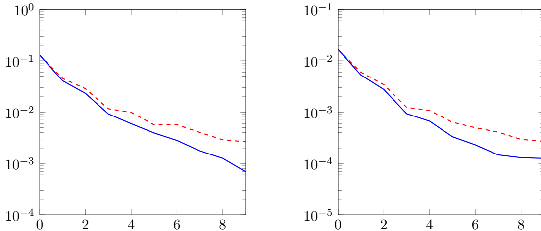
Figure 7.5: Plot of the error \|\varphi_1(\tau \mathbf{A}) \mathbf{A} \mathbf{y}_0 - \varphi_1(\tau \mathbf{A}_m) \mathbf{A} \mathbf{y}_0\|_{\mathbf{B}} versus m for the rational Krylov subspaces \mathcal{Q}_{2m+2}(\tau \mathbf{A}, \mathbf{A} \mathbf{y}_0) (blue solid line) and \mathcal{K}_{2m+2}((\gamma \mathbf{I} - \tau \mathbf{A})^{-1}, \mathbf{A} \mathbf{y}_0) for \tau = 0.05 and a mesh with 18 816 triangles, 10 057 nodes (left), \tau = 0.01 and a mesh with 301 056 triangles, 153 121 nodes (right), and parameters \gamma = 3 , h = 1 .
