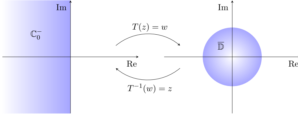
Figure 5.1: Transformation of the left complex half-plane \mathbb{C}_0^- onto the unit disk \overline{\mathbb{D}} \setminus \{-1\} and vice versa.
