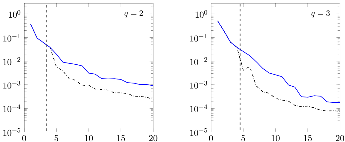
Figure 6.9: Comparison of the extended Krylov subspace approximation in \mathcal{K}_{q+1,m}^\gamma(\tau \mathbf{A}, \mathbf{y}_0^q) with N = 1\,046\,529 for q = 2 , \gamma = 1 (blue solid line), \gamma = 18^{3/5} (black dash-dotted line) on the left and q = 3 , \gamma = 1 (blue solid line), \gamma = 17^{5/11} (black dash-dotted line) on the right. The error \|e^{\tau \mathbf{A}} \mathbf{y}_0^q - e^{\tau \mathbf{A}_{q+m}} \mathbf{y}_0^q\|_{\mathbf{M}} is plotted versus the dimension of the extended Krylov subspace for \tau = 0.005 .
