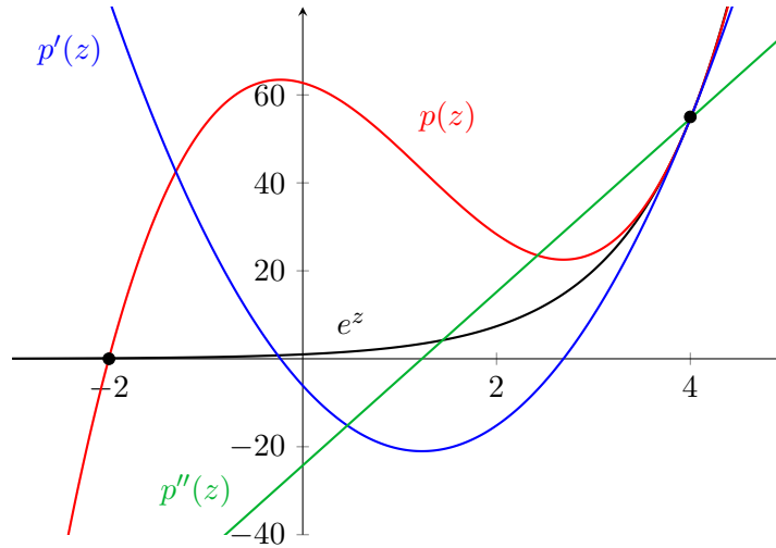
Figure 2.1: The exponential function and its Hermite interpolation polynomial p corresponding to the matrix \mathbf{A} .
