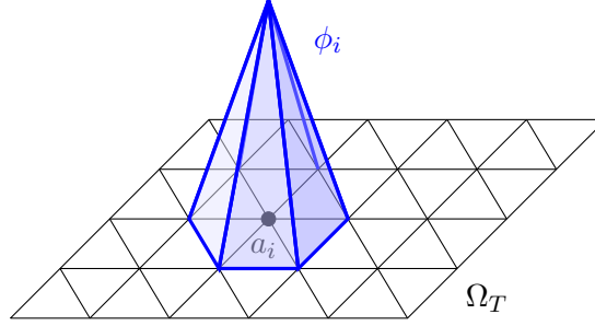
Figure 3.2: Basis function \phi_i corresponding to the node a_i .
