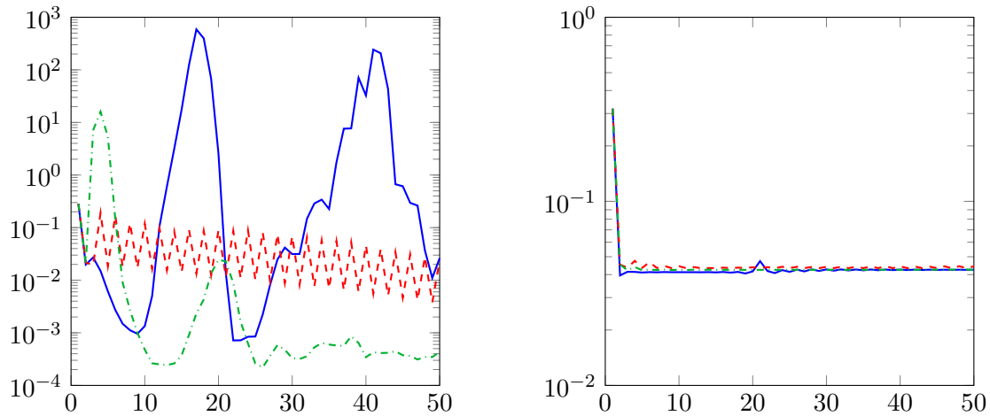
Figure 6.17: Plot of the error \|e^{\tau \mathbf{A}} \mathbf{y}_0^q - e^{\tau \mathbf{A}_{q+m}} \mathbf{y}_0^q\|_{\tilde{\mathbf{B}}} versus the dimension of the Krylov subspace for the standard Krylov subspace \mathcal{K}_{q+m,1}^\gamma(\tau \mathbf{A}, \mathbf{y}_0^q) (red dashed line), the rational Krylov subspace \mathcal{K}_{1,q+m}^\gamma(\tau \mathbf{A}, \mathbf{y}_0^q) (green dash-dotted line), and the extended Krylov subspace \mathcal{K}_{q+1,m}^\gamma(\tau \mathbf{A}, \mathbf{y}_0^q) (blue solid line) for the grid with 153 121 nodes, 301 056 triangles (left) and with 607 297 nodes, 1 204 224 triangles (right) for q = 1 , \gamma = 15 , \tau = 0.1 , and the “wrong” inner product with respect to \tilde{\mathbf{B}} = \text{diag}(\mathbf{M}, \mathbf{M}) .
