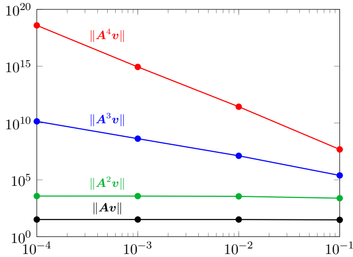
Figure 6.3: Plot of the discrete L^2 -norm \|A^j v\| for j = 1, \dots, 4 against the mesh size h .
