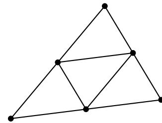
Figure 6.12: Refinement into 4 sub-triangles.
