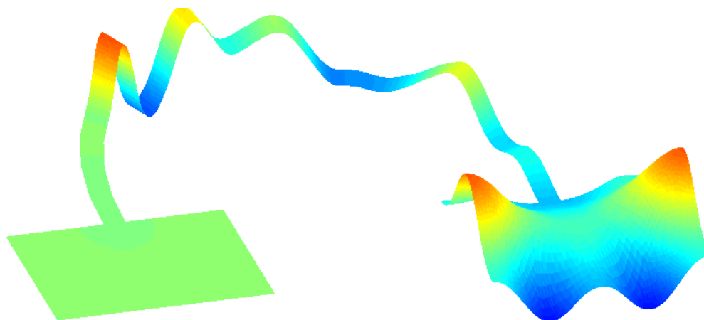
Figure 6.18: Approximation to the exact solution u at time \tau = 5 .
