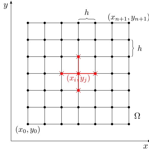
Figure 3.1: Two-dimensional grid for the finite-difference method on a square.
