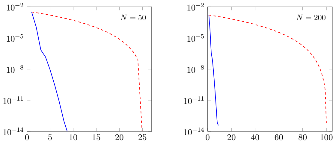
Figure 1.1: Comparison of the polynomial (red dashed line) and the rational (blue solid line) Krylov subspace method with N = 50, 200 discretization points.
