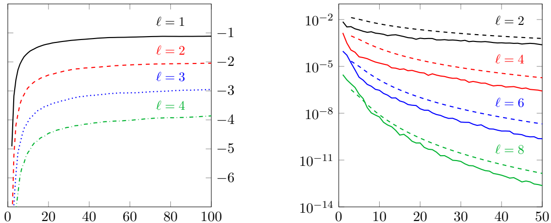
Figure 7.4: Left-hand side: Plot of \ln(E_m)/\ln(m) versus m for \gamma = 2 , h = 0.5 . Right-hand side: Plot of the error E_m for the rational Krylov subspace method with simple poles of distance h = \frac{\pi}{\ell}W(\frac{\pi m}{\ell})^{-1} and shift \gamma = 1 together with curves of order \mathcal{O}(\ln(m)^\ell/m^\ell) .
