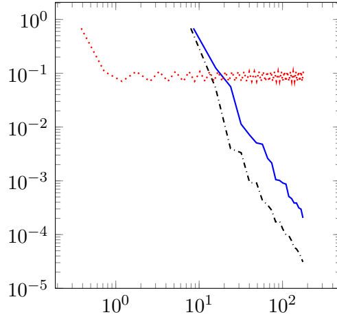
Figure 5.6: Plot of error versus computation time in seconds for the standard (red dotted line) and the shift-and-invert Krylov subspace method with \gamma = 1 (blue solid line) and \gamma = 20^{3/5} (black dash-dotted line) for N = 1\,048\,575 and \tau = 0.1 .
