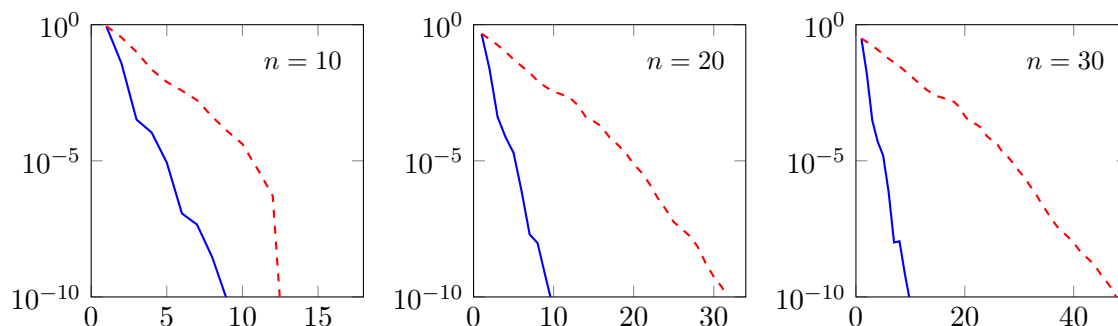
Figure 4.3: Plot of error versus iteration steps of the standard (red dashed line) and the rational (blue solid line) Krylov subspace method for the two-dimensional heat equation and n = 10, 20, 30 .
