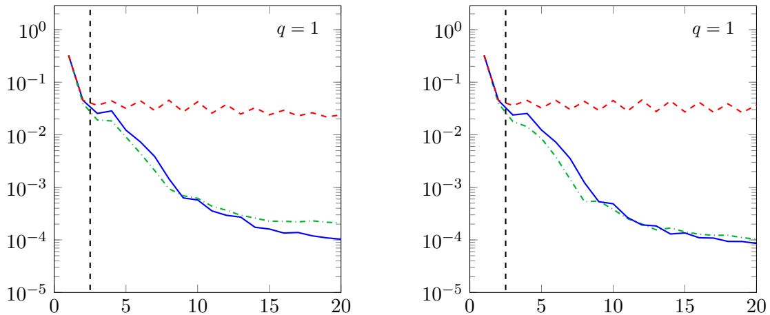
Figure 6.16: Plot of the error \|e^{\tau \mathbf{A}} \mathbf{y}_0^q - e^{\tau \mathbf{A}_{q+m}} \mathbf{y}_0^q\|_{\mathcal{B}} versus the dimension of the Krylov space for the standard Krylov subspace \mathcal{K}_{q+m,1}^{\gamma}(\tau \mathbf{A}, \mathbf{y}_0^q) (red dashed line), the rational Krylov subspace \mathcal{K}_{1,q+m}^{\gamma}(\tau \mathbf{A}, \mathbf{y}_0^q) (green dash-dotted line), and the extended Krylov subspace \mathcal{K}_{q+1,m}^{\gamma}(\tau \mathbf{A}, \mathbf{y}_0^q) (blue solid line) for fine grids with 153 121 nodes, 301 056 triangles (left) and with 607 297 nodes, 1 204 224 triangles (right) for q = 1 , \gamma = 15 , and \tau = 0.1 .
