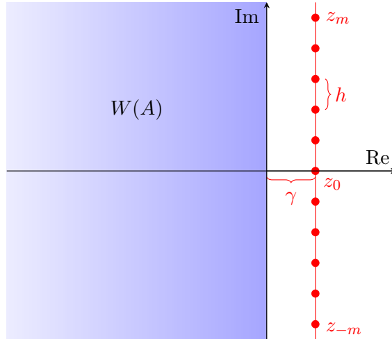
Figure 7.1: Locus of W(\mathbf{A}) and the roots z_k of the denominator polynomial q_{2m+1} .
