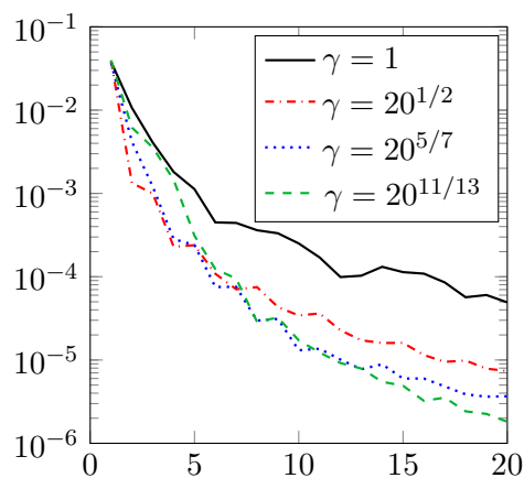
Figure 5.3: Error \|\varphi_4(\mathbf{A})\mathbf{v} - \varphi_4(\mathbf{A}_m)\mathbf{v}\| versus m .
