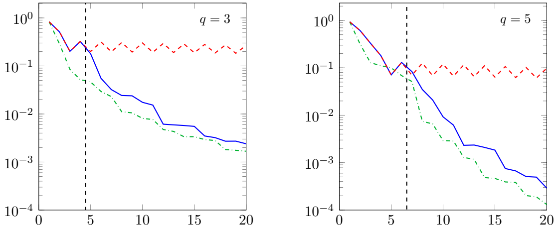
Figure 6.5: Plot of the error \|e^{\tau \mathbf{A}} \tilde{\mathbf{y}}_0^q - e^{\tau \mathbf{A}_{q+m}} \tilde{\mathbf{y}}_0^q\|_2 versus the dimension of the Krylov subspace for the standard Krylov subspace \mathcal{K}_{q+m,1}^\gamma(\tau \mathbf{A}, \tilde{\mathbf{y}}_0^q) (red dashed line), the rational Krylov subspace \mathcal{K}_{1,q+m}^\gamma(\tau \mathbf{A}, \tilde{\mathbf{y}}_0^q) (green dash-dotted line), and the extended Krylov subspace \mathcal{K}_{q+1,m}^\gamma(\tau \mathbf{A}, \tilde{\mathbf{y}}_0^q) (blue solid line) with initial vectors \tilde{\mathbf{y}}_0^q , q = 3, 5 , whose continuous counterparts satisfy \tilde{\mathbf{y}}_0^q \in D(A^q) but \tilde{\mathbf{y}}_0^q \notin D(A^{q+1}) . The parameters are chosen as \gamma = 1 , \tau = 0.1 , and N = 1023 .
