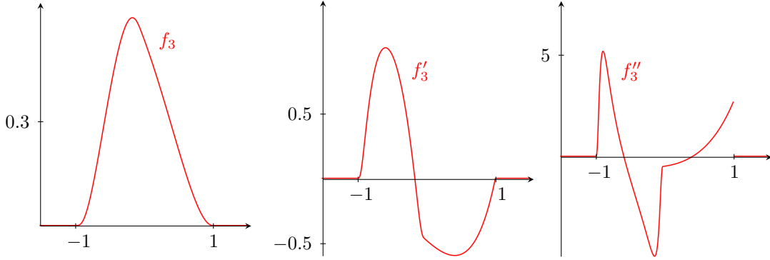
Figure 7.2: Plot of f_3 , f'_3 , and the weak derivative f''_3 with jump discontinuity at 1.
