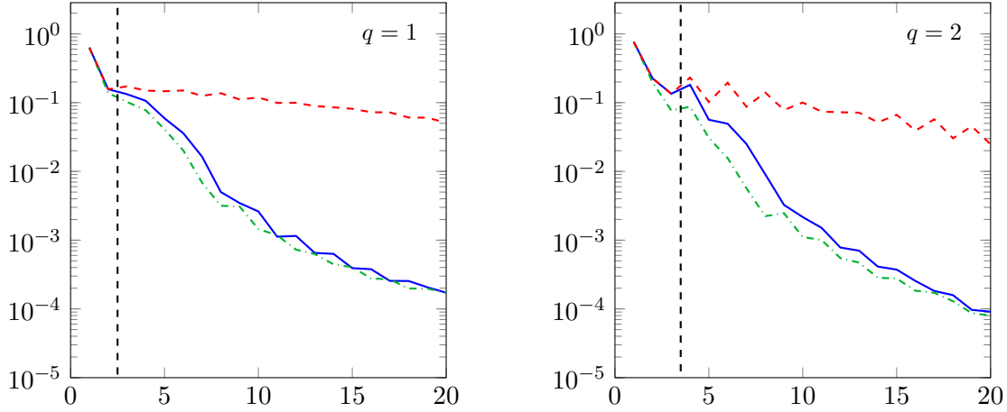
Figure 6.15: Plot of the error \|e^{\tau\mathbf{A}}\mathbf{y}_0^q - e^{\tau\mathbf{A}_{q+m}}\mathbf{y}_0^q\|_{\mathbf{B}} versus the dimension of the Krylov subspace for the standard Krylov subspace \mathcal{K}_{q+m,1}^\gamma(\tau\mathbf{A}, \mathbf{y}_0^q) (red dashed line), the rational Krylov subspace \mathcal{K}_{1,q+m}^\gamma(\tau\mathbf{A}, \mathbf{y}_0^q) (green dash-dotted line), and the extended Krylov subspace \mathcal{K}_{q+1,m}^\gamma(\tau\mathbf{A}, \mathbf{y}_0^q) (blue solid line) for a coarse grid with 18 816 triangles, 10 057 nodes, \gamma = 15 , \tau = 0.1 , and smoothness indices q = 1, 2 .
