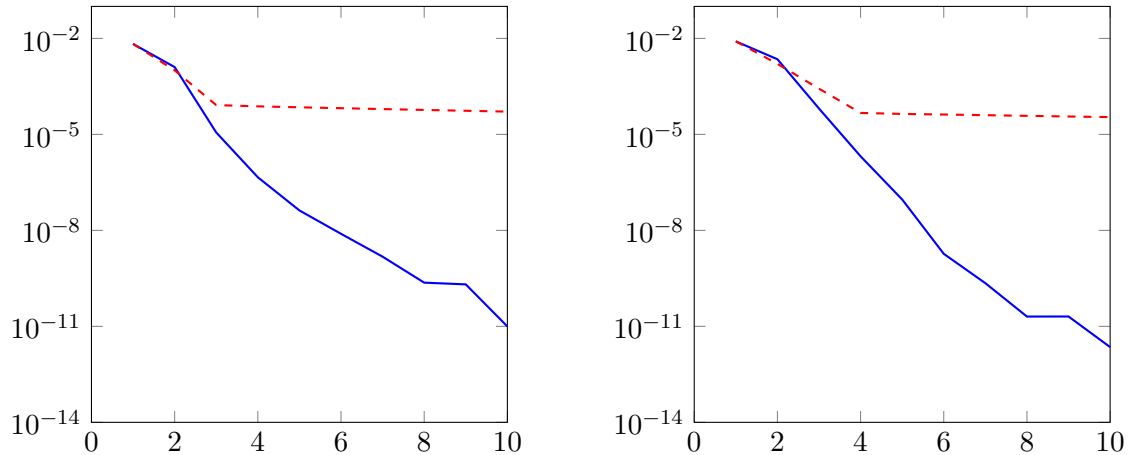
Figure 1.2: Convergence of the polynomial (red dashed line) and the rational (blue solid line) Krylov subspace approximation for the initial values u_0(x) = x^6(1-x)^6 (left) and u_0(x) = x^8(1-x)^8 (right).
