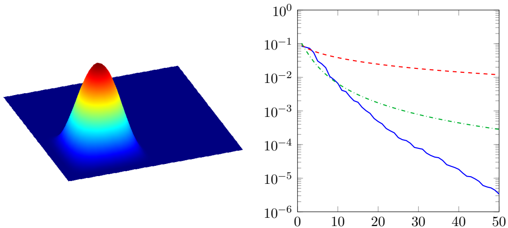
Figure 5.7: Left-hand side: Initial value u_0 on the unit square. Right-hand side: Plot of the approximation error E_m versus m (blue solid line) together with the error of the implicit Euler method (red dashed line) and the Crank-Nicolson scheme (green dash-dotted line).
