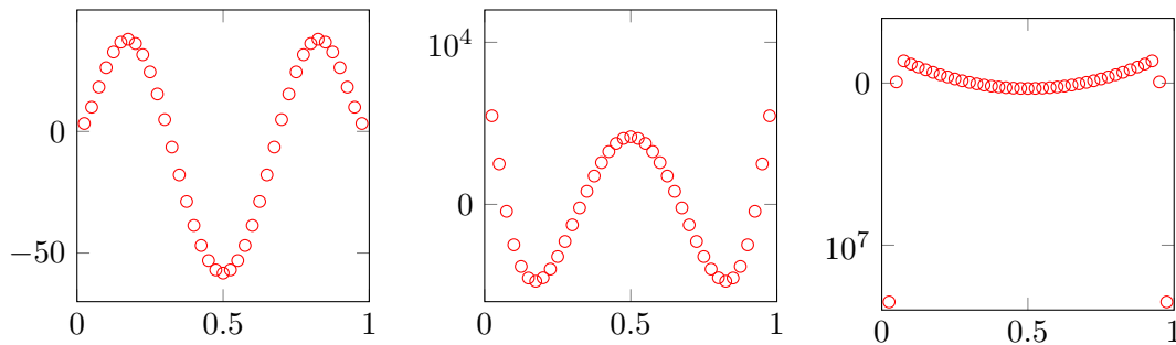
Figure 6.1: Plot of \mathbf{A}\mathbf{v} , \mathbf{A}^2\mathbf{v} and \mathbf{A}^3\mathbf{v} for N = 39 .
