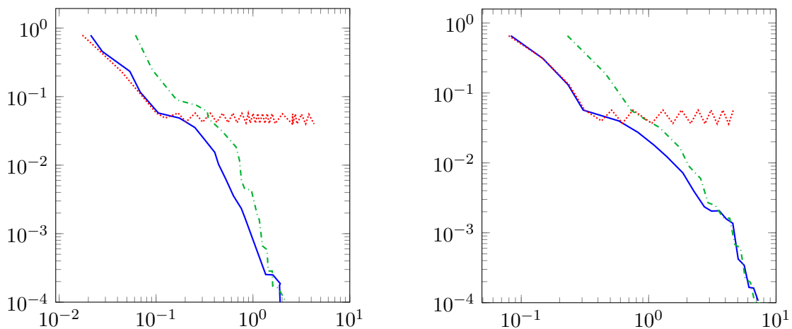
Figure 6.8: Plot of error versus computation time in seconds for the standard (red dotted line), the rational (green dash-dotted line) and the extended (blue solid line) Krylov subspace method for q = 5 , N = 65\,025 on the left-hand side and q = 4 , N = 261\,121 on the right-hand side as well as \gamma = 1 , \tau = 0.005 in both cases.
