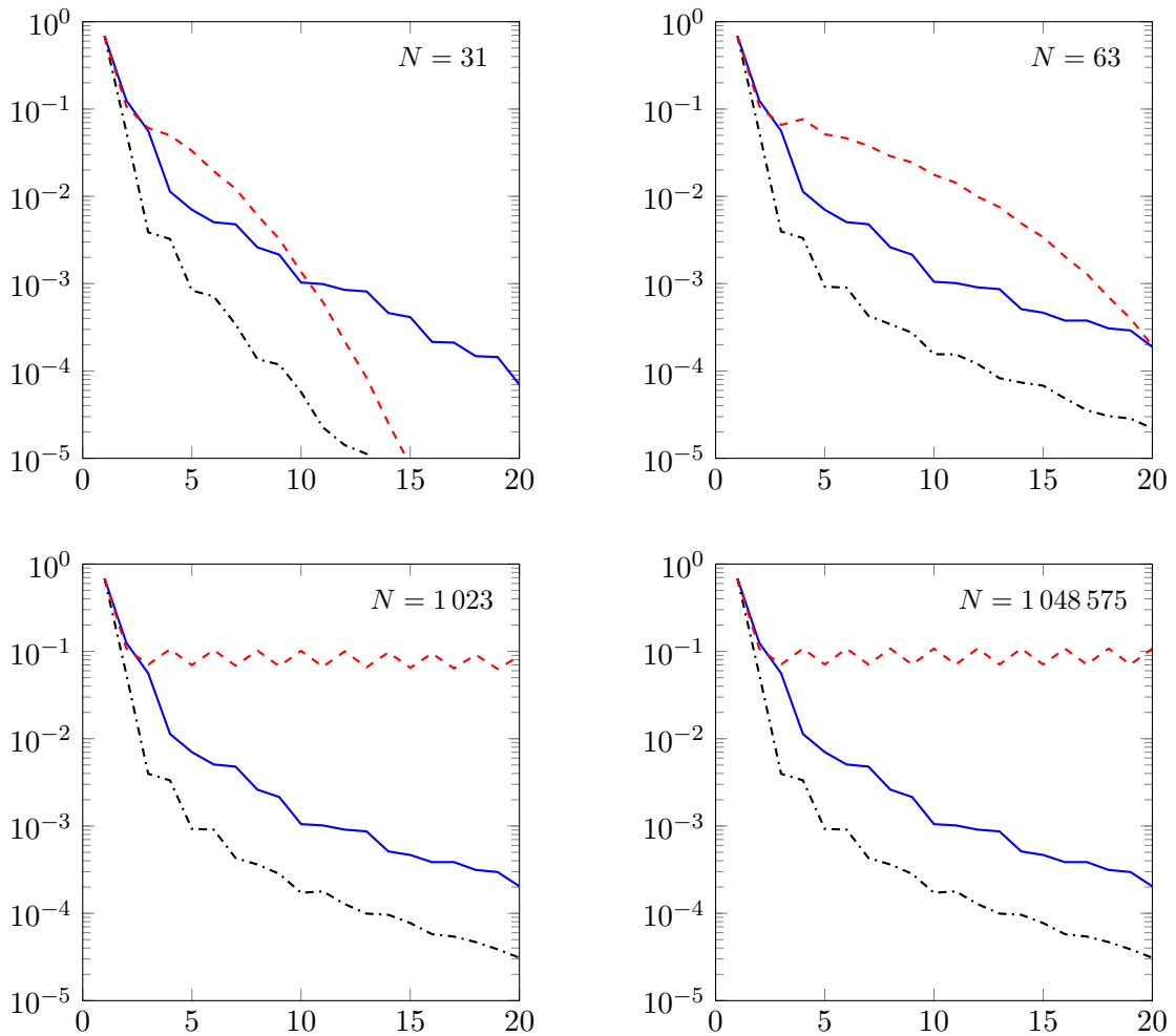
Figure 5.5: Plot of the error \|\varphi_1(\tau\mathbf{A})(\mathbf{A}\mathbf{y}_0 + \mathbf{F}) - \varphi_1(\tau\mathbf{A}_m)(\mathbf{A}\mathbf{y}_0 + \mathbf{F})\|_2 versus the dimension of the Krylov subspace for the standard Krylov subspace \mathcal{K}_m(\tau\mathbf{A}, \mathbf{A}\mathbf{y}_0 + \mathbf{F}) (red dashed line) and the shift-and-invert Krylov subspace \mathcal{Q}_m(\tau\mathbf{A}, \mathbf{A}\mathbf{y}_0 + \mathbf{F}) with \gamma = 1 (blue solid line) and \gamma = 20^{3/5} (black dash-dotted line) for \tau = 0.1 , N = 31, 63, 1023, 1048575 .
