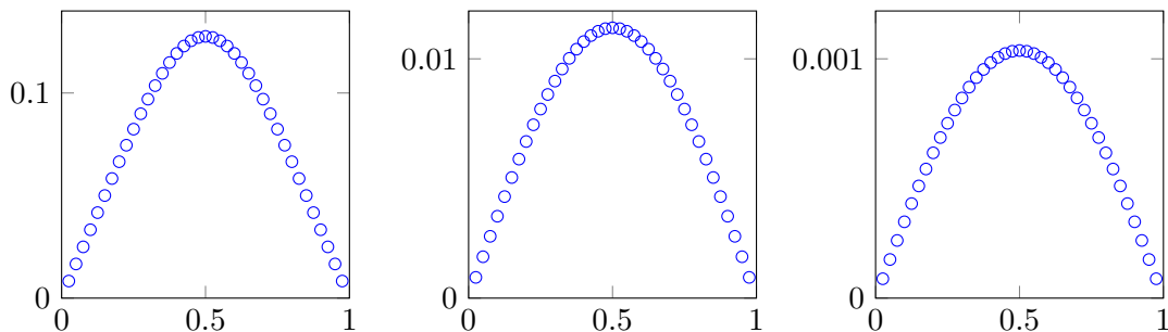
Figure 6.2: Plot of (\gamma\mathbf{I} - \mathbf{A})^{-1}\mathbf{v} , (\gamma\mathbf{I} - \mathbf{A})^{-2}\mathbf{v} and (\gamma\mathbf{I} - \mathbf{A})^{-3}\mathbf{v} for \gamma = 1 and N = 39 .
