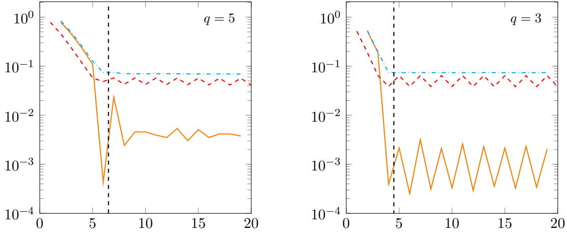
Figure 6.11: Plot of E_m (cyan dash-dotted line) and \tilde{E}_m (orange solid line) versus m together with the error \|e^{\tau A} \mathbf{y}_0^q - e^{\tau A_m} \mathbf{y}_0^q\|_M of the standard Krylov subspace approximation (red dashed line) for N = 65\,025 , q = 5 (left), N = 1\,046\,529 , q = 3 (right), and \tau = 0.005 .
