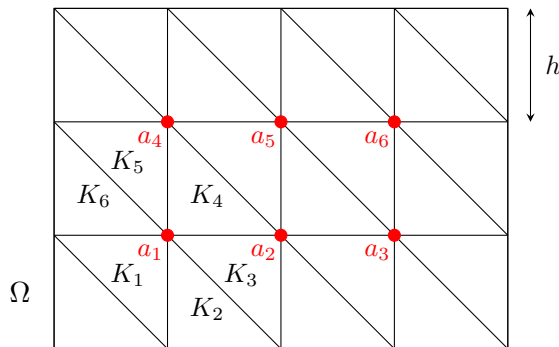
Figure 3.3: Regular grid used in Example 3.1.
