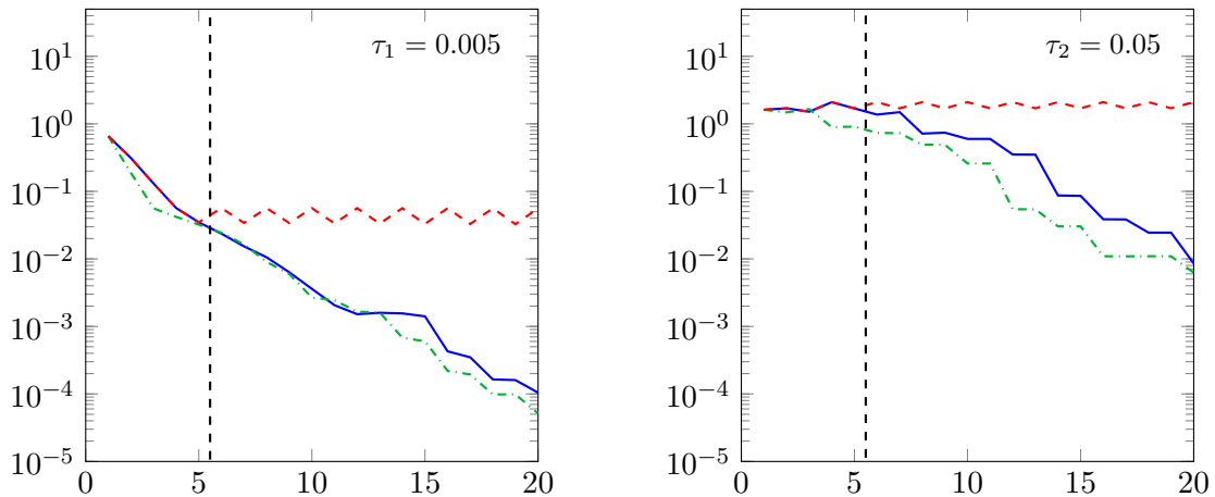
Figure 6.10: Plot of the error \|e^{\tau_i \mathbf{A}} \mathbf{y}_0^4 - e^{\tau_i \mathbf{A}_{q+m}} \mathbf{y}_0^4\|_{\mathbf{M}} versus the dimension of the Krylov subspace for the standard Krylov subspace \mathcal{K}_{q+m,1}^\gamma(\tau_i \mathbf{A}, \mathbf{y}_0^4) (red dashed line), the rational Krylov subspace \mathcal{K}_{1,q+m}^\gamma(\tau_i \mathbf{A}, \mathbf{y}_0^4) (green dash-dotted line) and the extended Krylov subspace \mathcal{K}_{q+1,m}^\gamma(\tau_i \mathbf{A}, \mathbf{y}_0^4) (blue solid line) with parameters N = 1\,046\,529 , \gamma = 1 , q = 4 , and time step sizes \tau_1 = 0.005 , \tau_2 = 0.05 .
