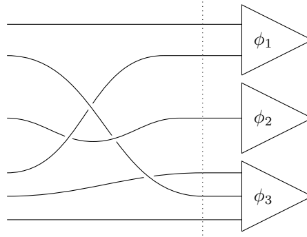
FIGURE 6. Arrow in \mathcal{S}(\mathcal{O}) .
