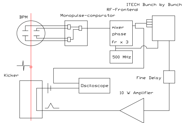
Figure 1: Schematic view of the bunch by bunch feedback set up.
