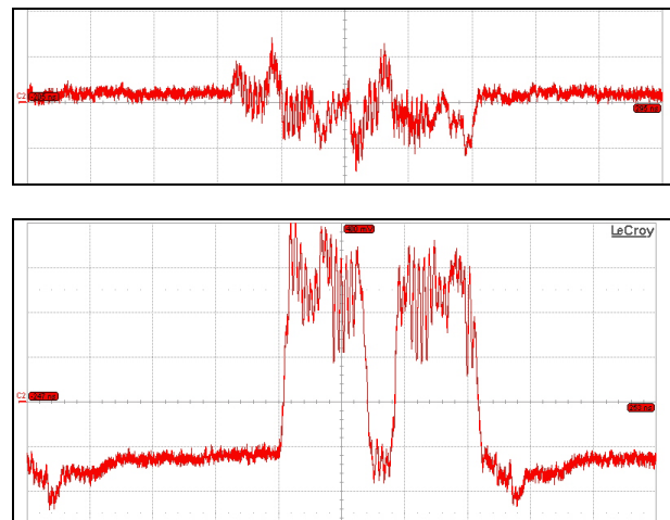
Figure 2: Scope signal for two trains from the RF front end while in frequency (upper graph) and amplitude modulation (lower graph) mode.
