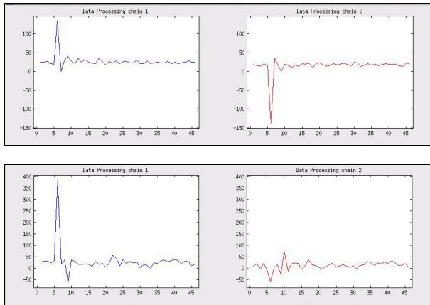
Figure 3: ADC signal of one bunch for incorrect clock timing (upper graph, the signal is distributed over two channels) and correct timing (lower graph).
