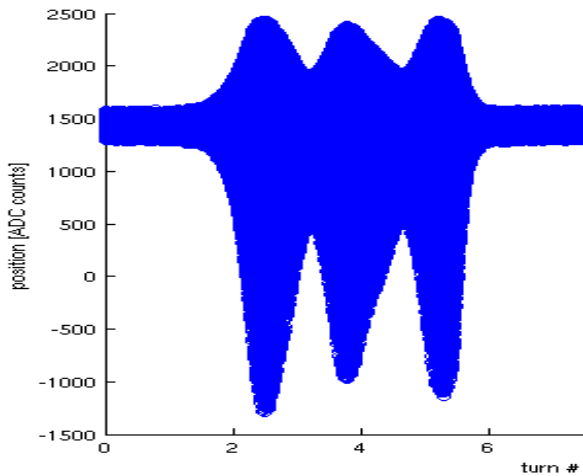
Figure 7: Vertical instabilities at a chromaticity of +3. Scale x10000 turns.
