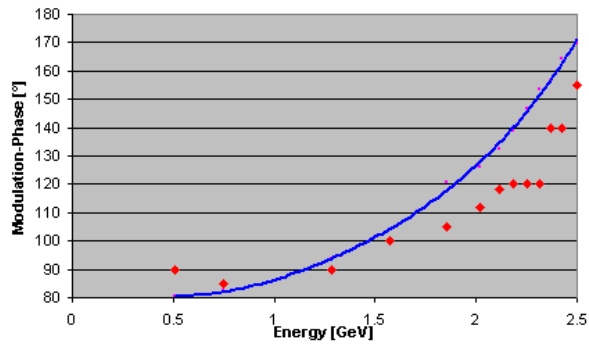
Figure 6: Behaviour of phase during ramping of energy.
