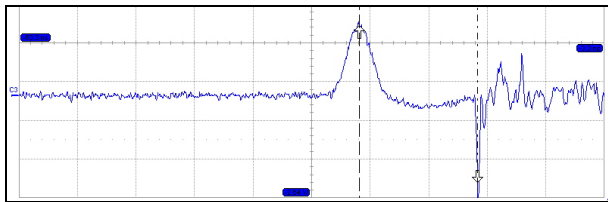
Figure 4: Signal from Kicker upstream port. Left peak from amplifier, right (needle) from bunch.
