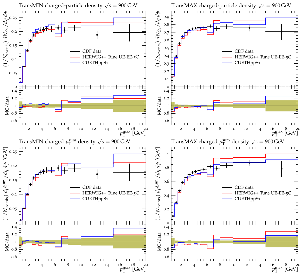
Fig. 28 CDF data at \sqrt{s} = 900 \text{ GeV} [11] on particle ( top ) and p_T^{\text{sum}} densities ( bottom ) for charged particles with p_T > 0.5 \text{ GeV} and |\eta| < 0.8 in the TransMIN ( left ) and TransMAX ( right ) regions as defined by the leading charged particle, as a function of the transverse momentum of
