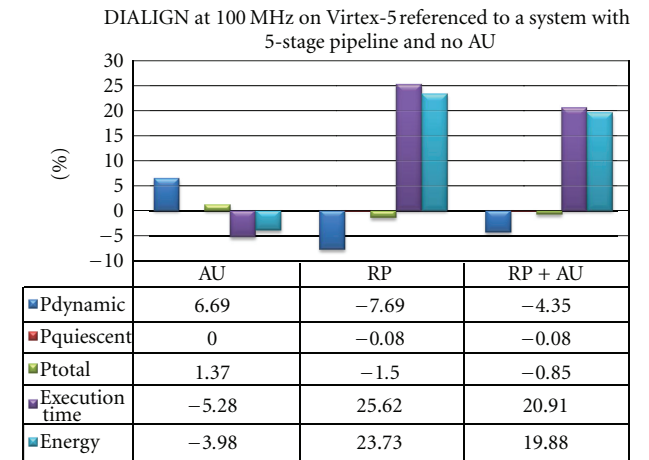
FIGURE 29: Impact of the MicroBlaze configurations for the DIALIGN algorithm.
