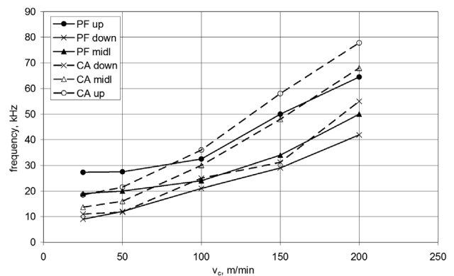
Figure 15: Influence of cutting speed on the peak frequency (PF) of the D9241A sensor and calculated segmentation frequency (CA) Slika 15: Vpliv hitrosti rezanja na maksimalno frekvenco (PF) senzorja D9241A in izračunana frekvenca segmentacije (CA)
