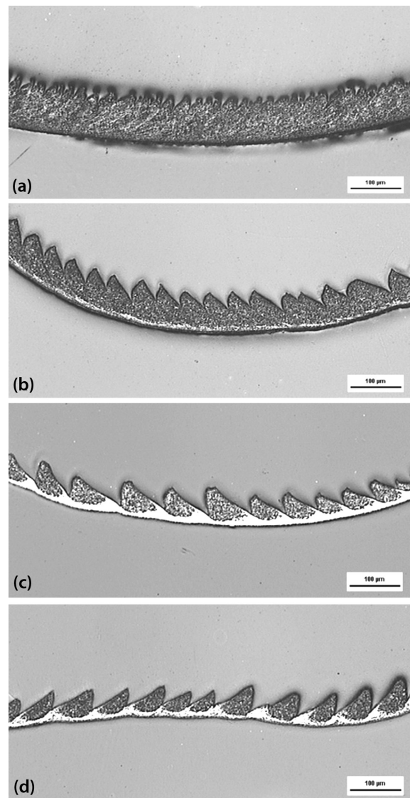
Figure 4: Chips after hard turning: a) v_c = 25 \text{ m min}^{-1} , f = 0.09 \text{ mm} , b) v_c = 50 \text{ m min}^{-1} , f = 0.09 \text{ mm} , c) v_c = 100 \text{ m min}^{-1} , f = 0.09 \text{ mm} , d) v_c = 200 \text{ m min}^{-1} , f = 0.09 \text{ mm}
