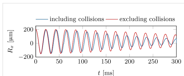
Figure 3: Center-of-mass oscillation of a cold-atom tip in an anharmonic potential with/without particle collisions (blue/red solid line). The simulation parameters have been chosen as before: T = 500 nK, N = 5 \times 10^5 atoms, \varepsilon = 2 \times 10^8 \text{ m}^{-1} \text{ s}^{-2} , (\omega_x, \omega_y, \omega_z) = 2\pi \times (50, 500, 500) Hz, A = 200 \text{ }\mu\text{m} .
