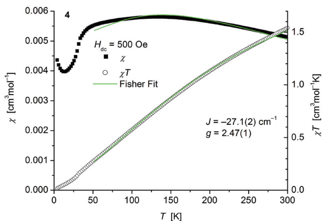
Fig. 8 Temperature dependence of \chi (filled squares) and \chi T (open circles) of \frac{1}{2}[\text{Co}(\text{SPh})_2(\text{NH}_3)] ( 4 ). Solid green lines represent the results of the fitting to Fisher's equation (eqn (1)).
